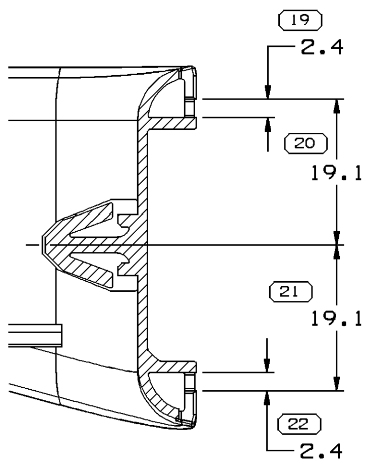
SECTION C-C
