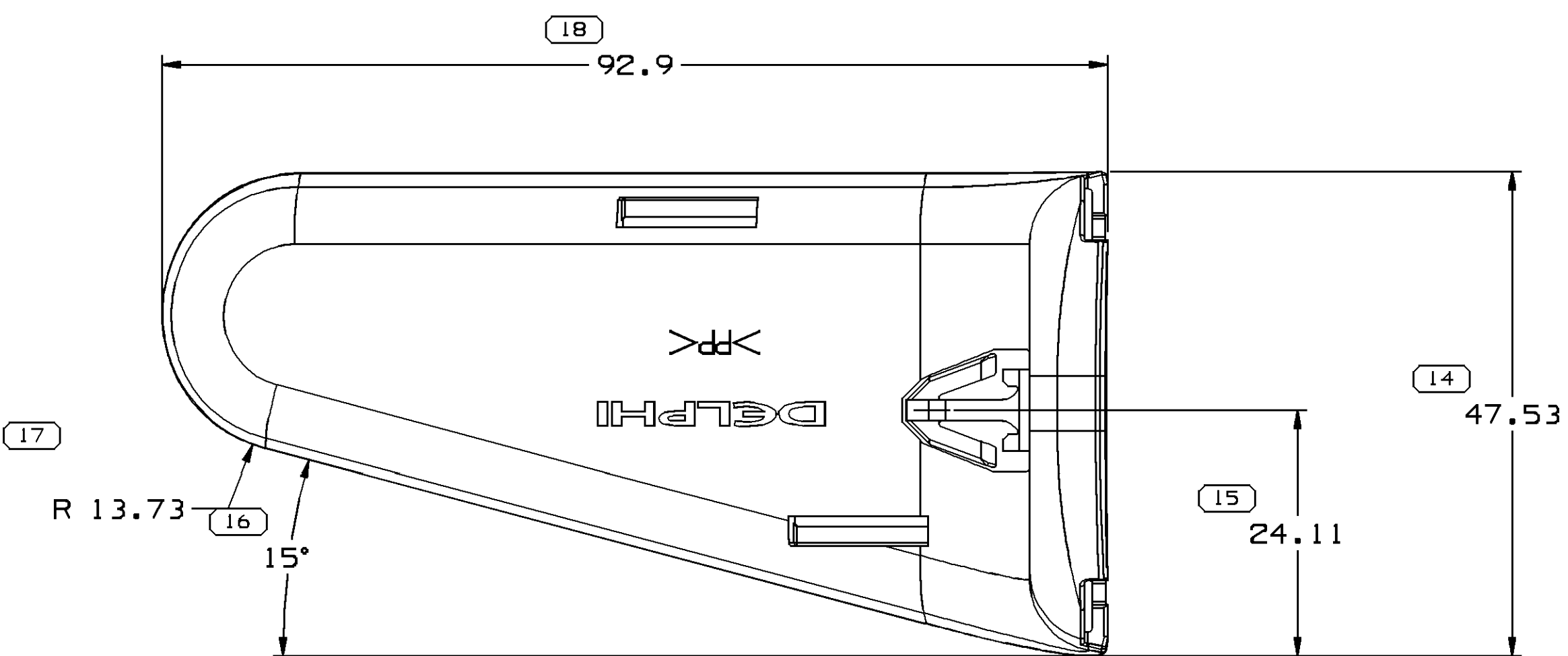
SECTION C-C
