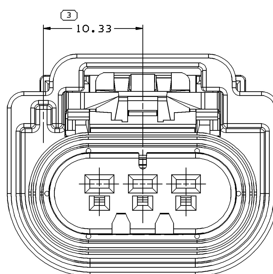
TYPE 208 SAME AS TYPE 202 EXCEPT AS SHOWN
