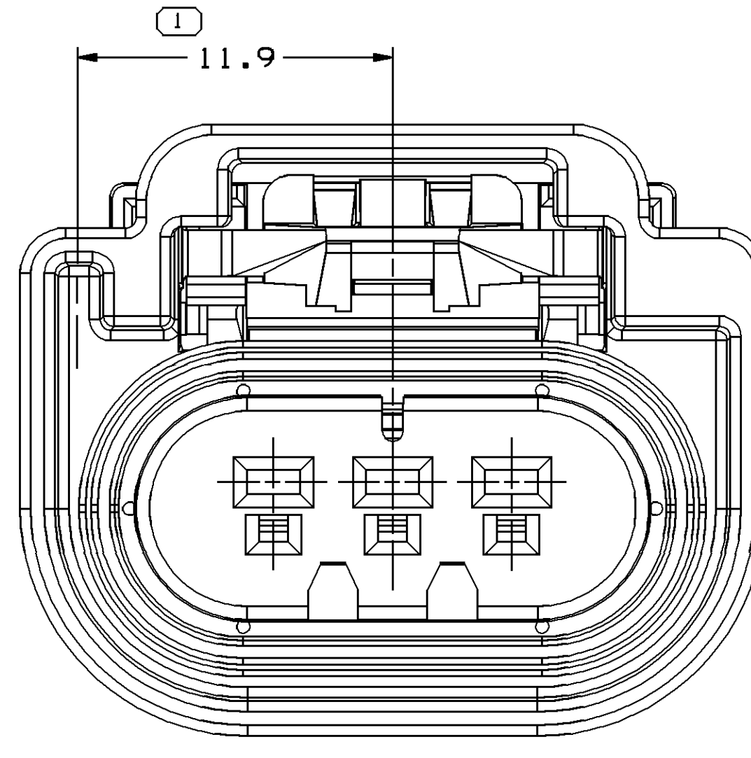
TYPE 210 SAME AS TYPE 201 EXCEPT AS SHOWN
