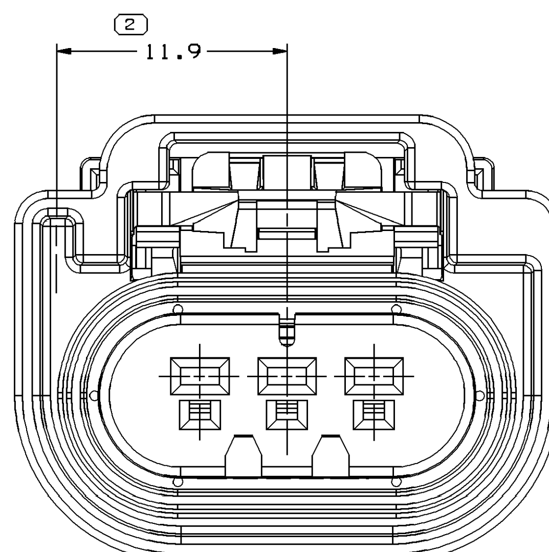
TYPE 209 SAME AS TYPE 202 EXCEPT AS SHOWN
