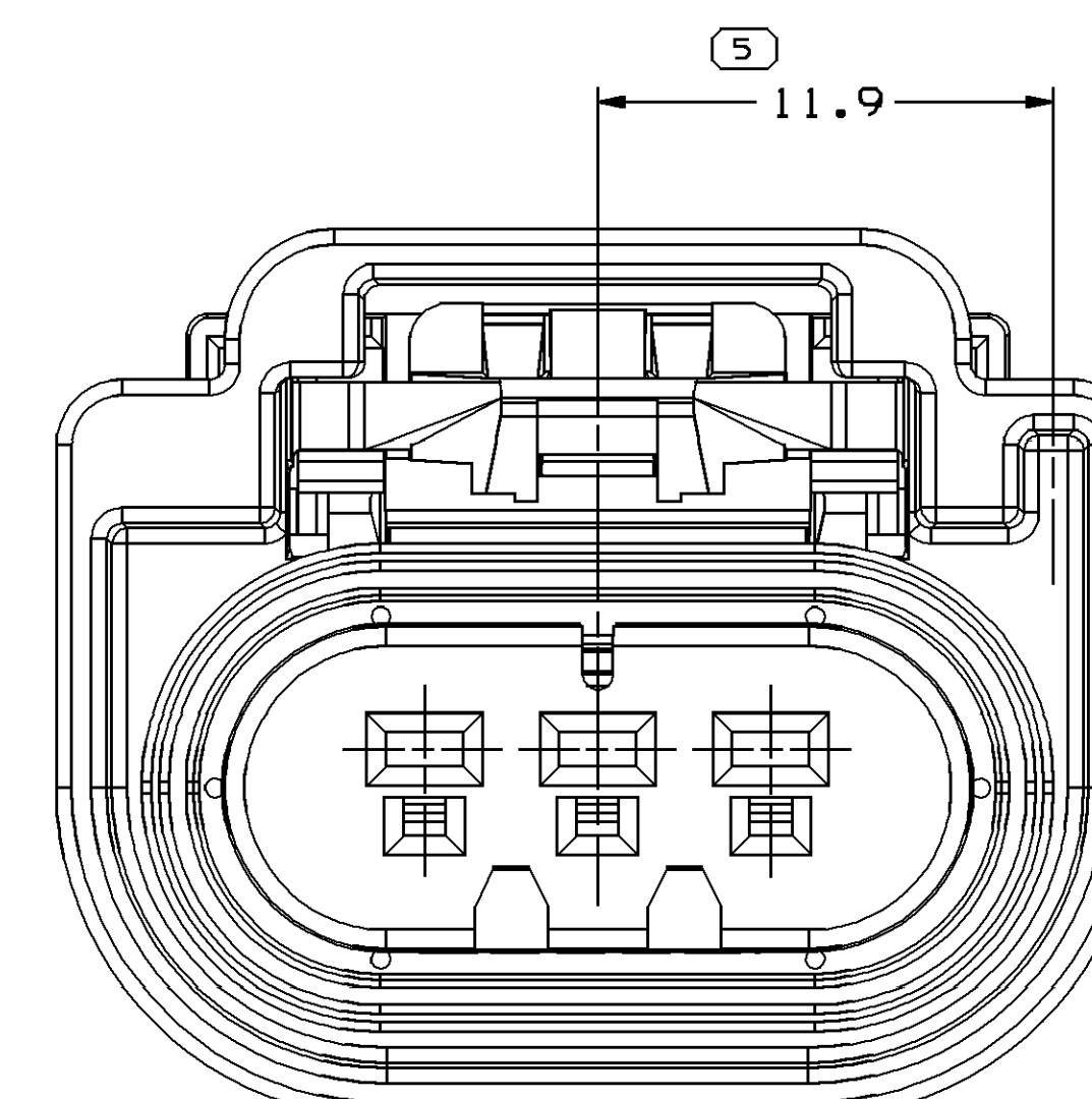
TYPE 206 SAME AS TYPE 202 EXCEPT AS SHOWN
