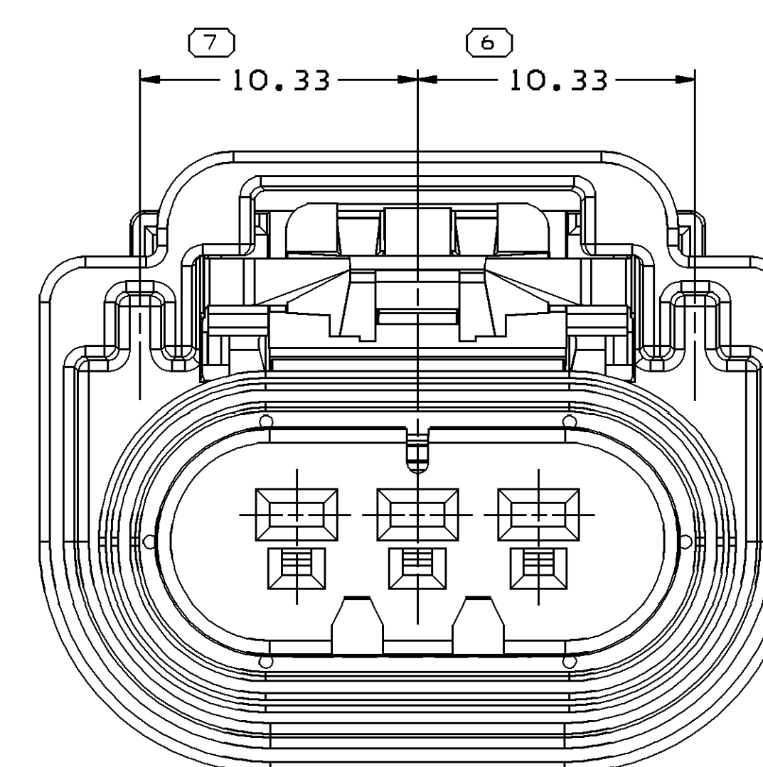
TYPE 205 SAME AS TYPE 202 EXCEPT AS SHOWN
