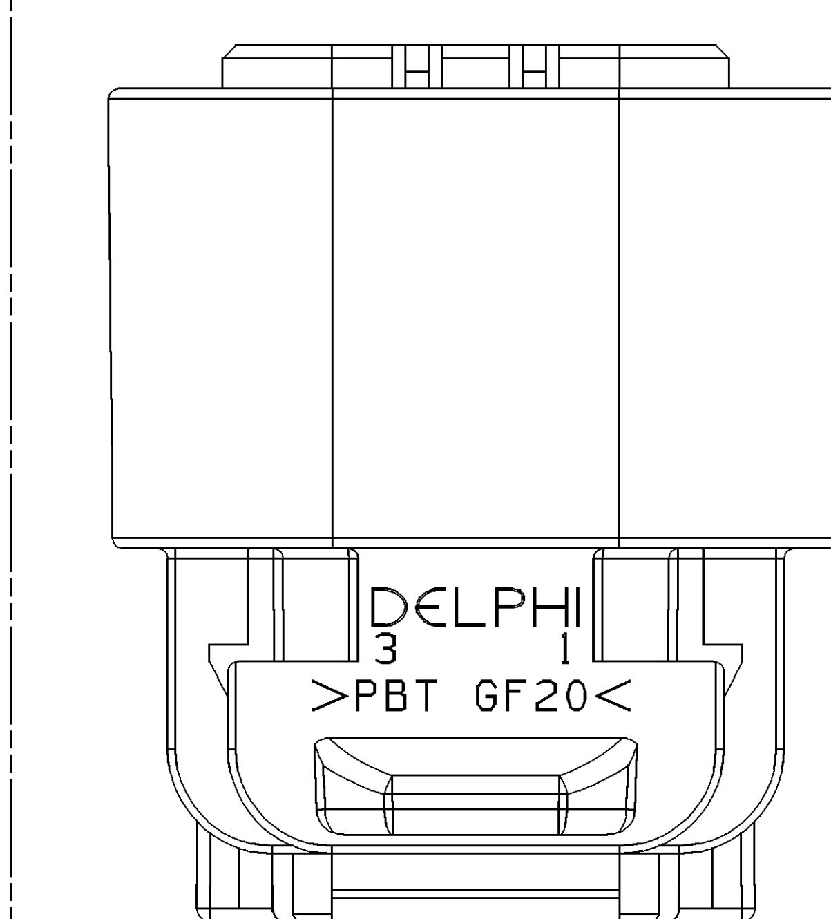
TYPE 202 SAME AS TYPE 201 EXCEPT MATL SPEC CALLOUT (SEE CHART) AND CAVITY IDENTIFICATION
