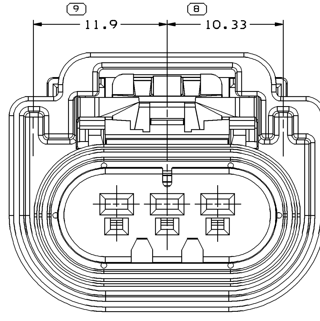
TYPE 204 SAME AS TYPE 202 EXCEPT AS SHOWN
