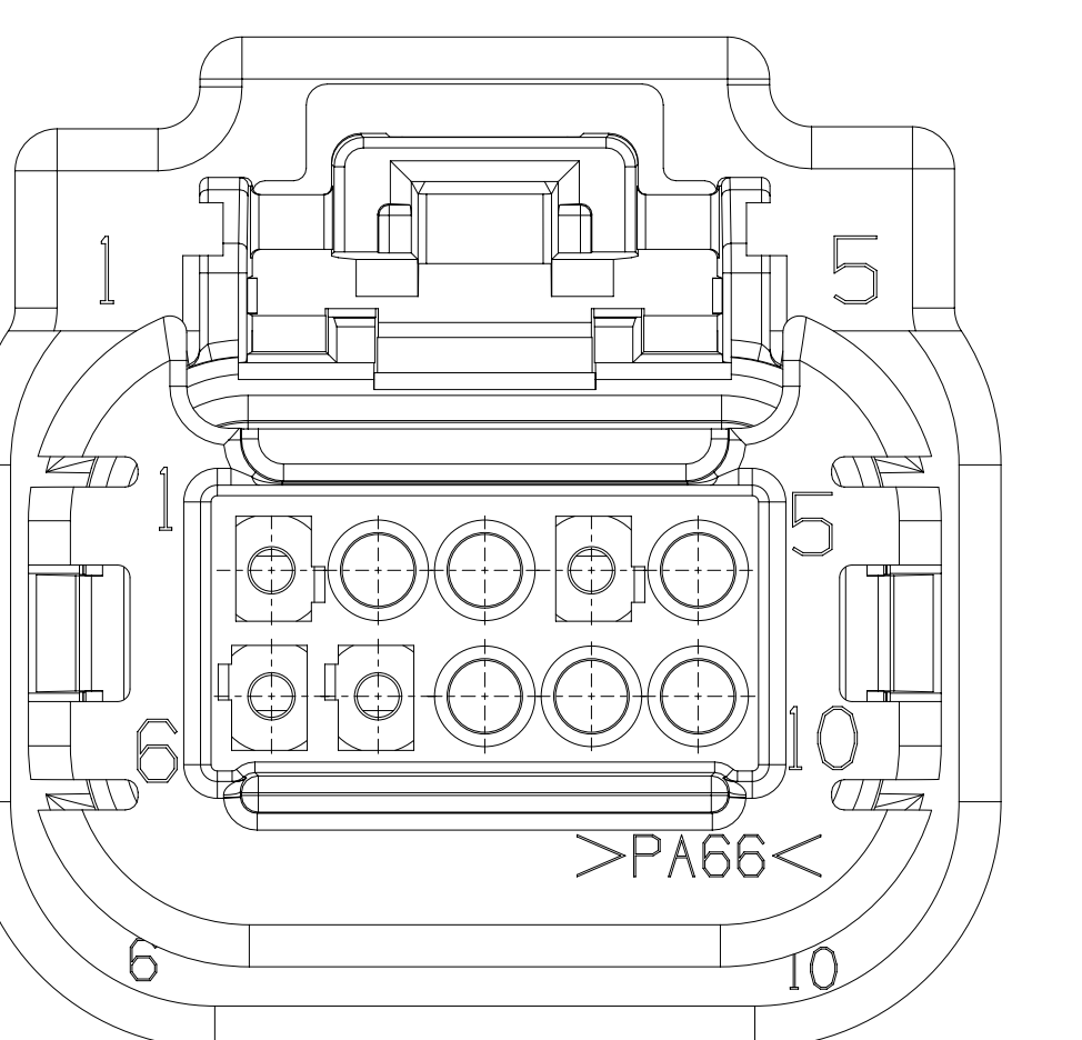
TYPE 210 SAME AS TYPE 201 EXCEPT AS SHOWN
