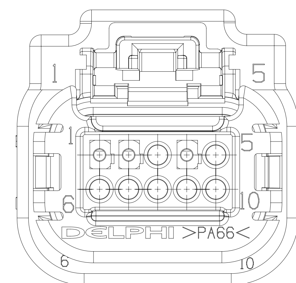
TYPE 202 SAME AS TYPE 20 EXCEPT AS SHOWN
