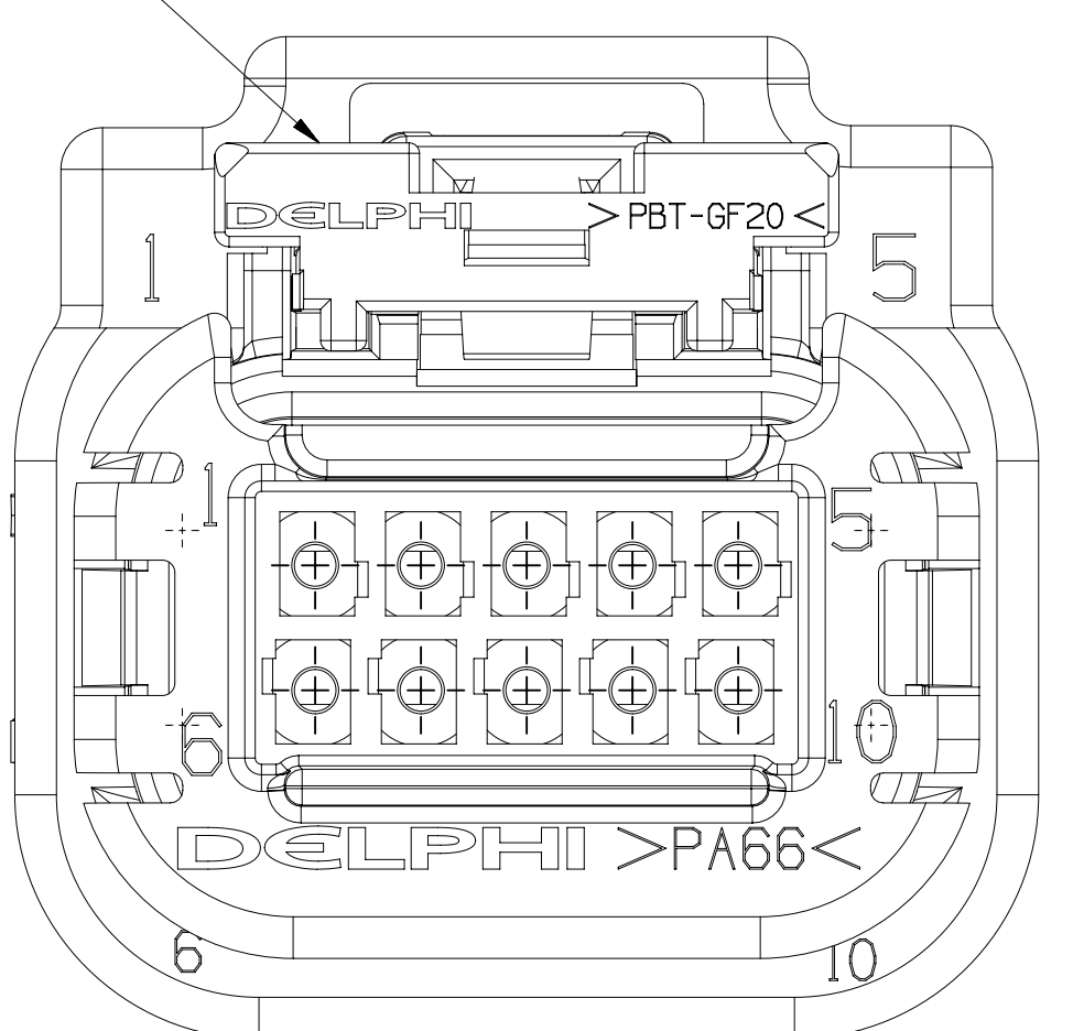
TYPE 208 SAME AS TYPE 205 EXCEPT AS SHOWN
