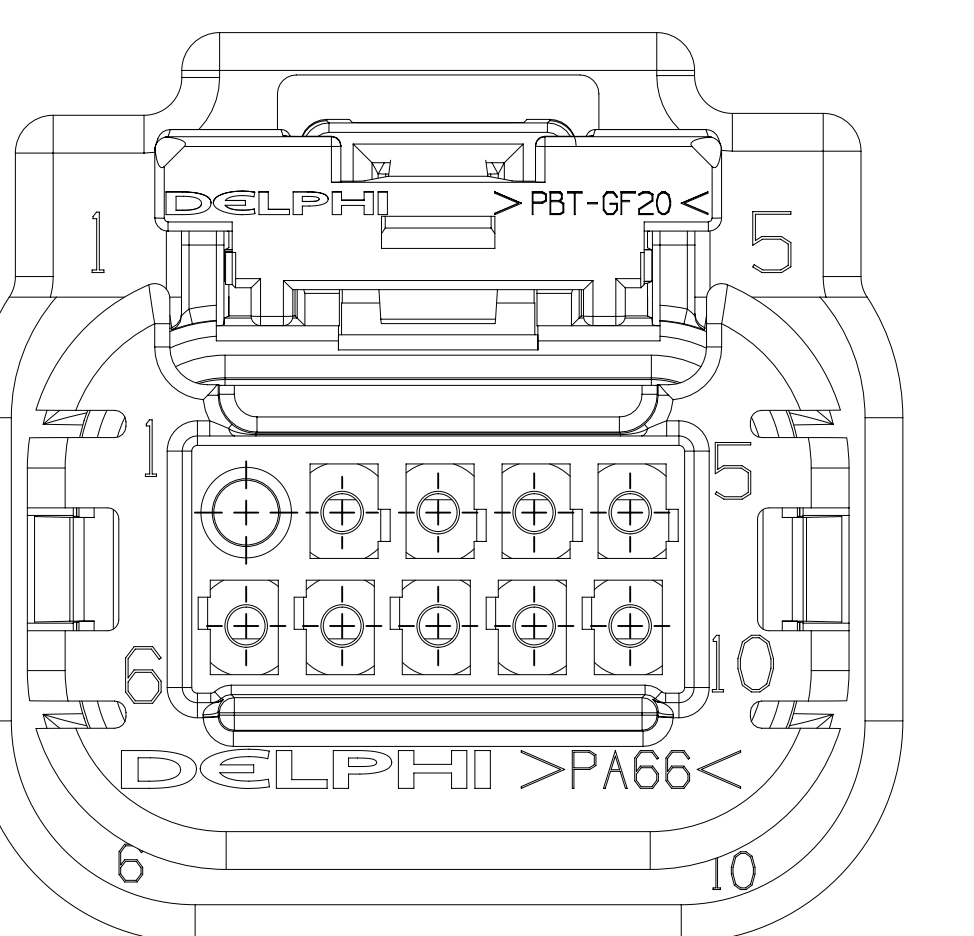
TYPE 209 SAME AS TYPE 201 EXCEPT AS SHOWN
