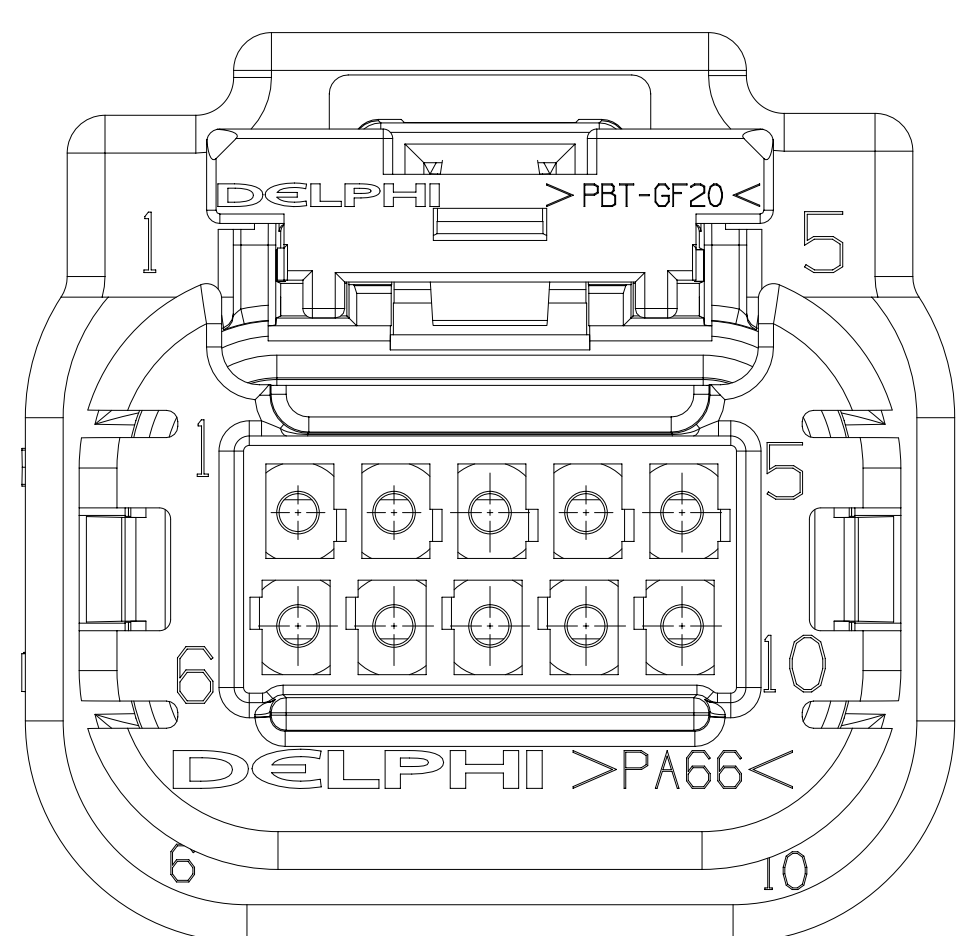
TYPE 205 SAME AS TYPE 203 EXCEPT AS SHOWN
