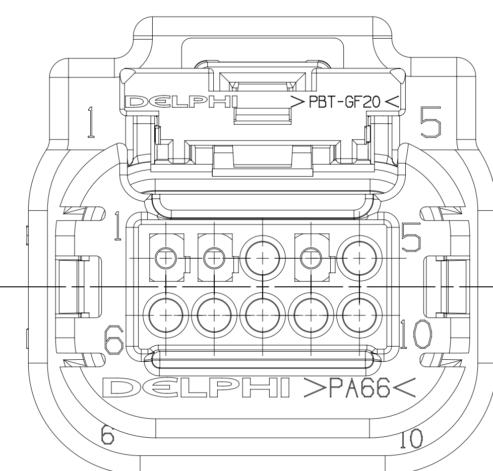
TYPE 203 SAME AS TYPE 202 EXCEPT AS SHOWN
