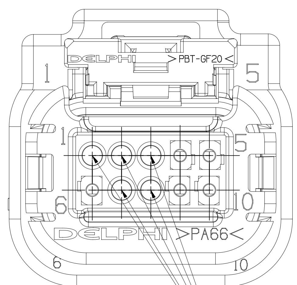
BLOCKED CAVITIES
