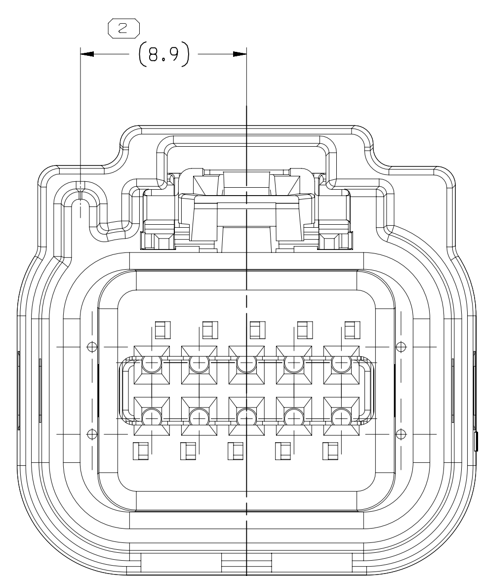
TYPE 103 SAME AS TYPE 101 EXCEPT AS SHOWN
