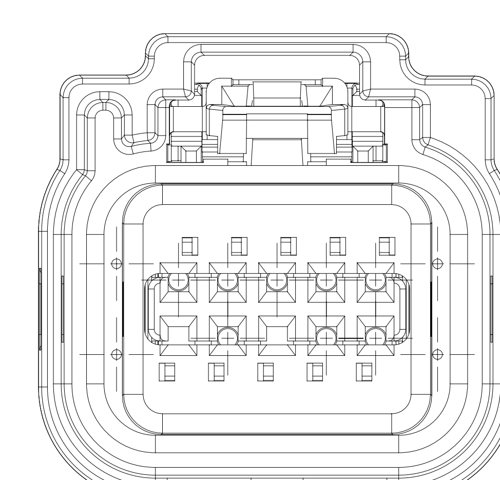
TYPE 106 SAME AS TYPE 103 EXCEPT AS SHOWN
