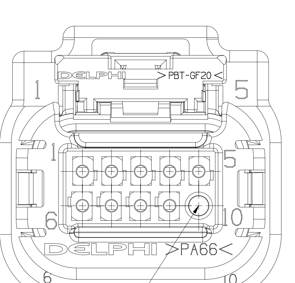
BLOCKED CAVITY
