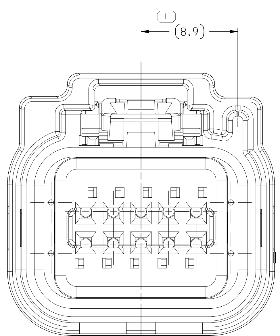
TYPE 102 SAME AS TYPE 101 EXCEPT AS SHOWN
