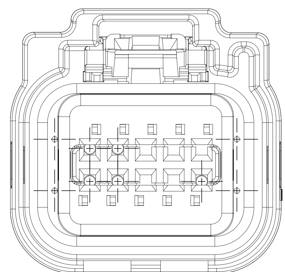
TYPE 112 SAME AS TYPE 102 EXCEPT AS SHOWN
