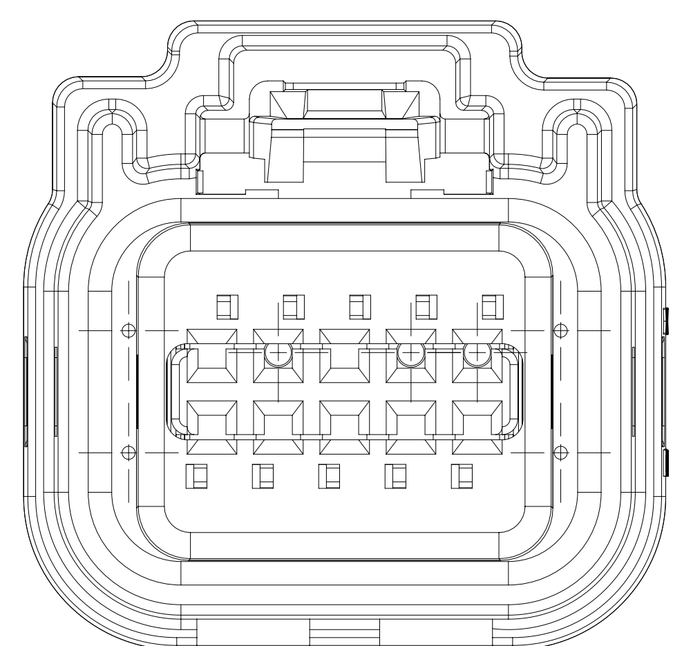
TYPE 108 SAME AS TYPE 101 EXCEPT AS SHOWN
