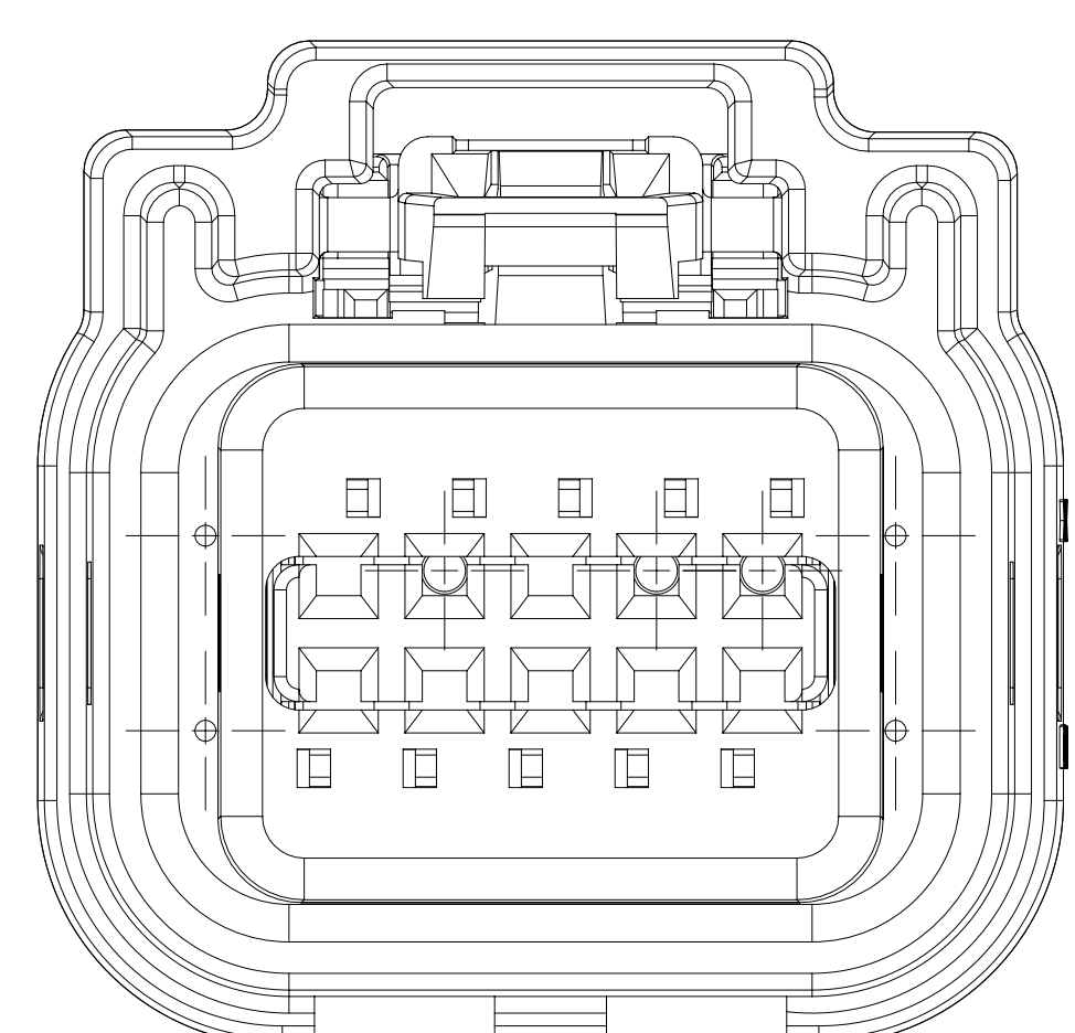
TYPE 109 SAME AS TYPE 101 EXCEPT AS SHOWN
