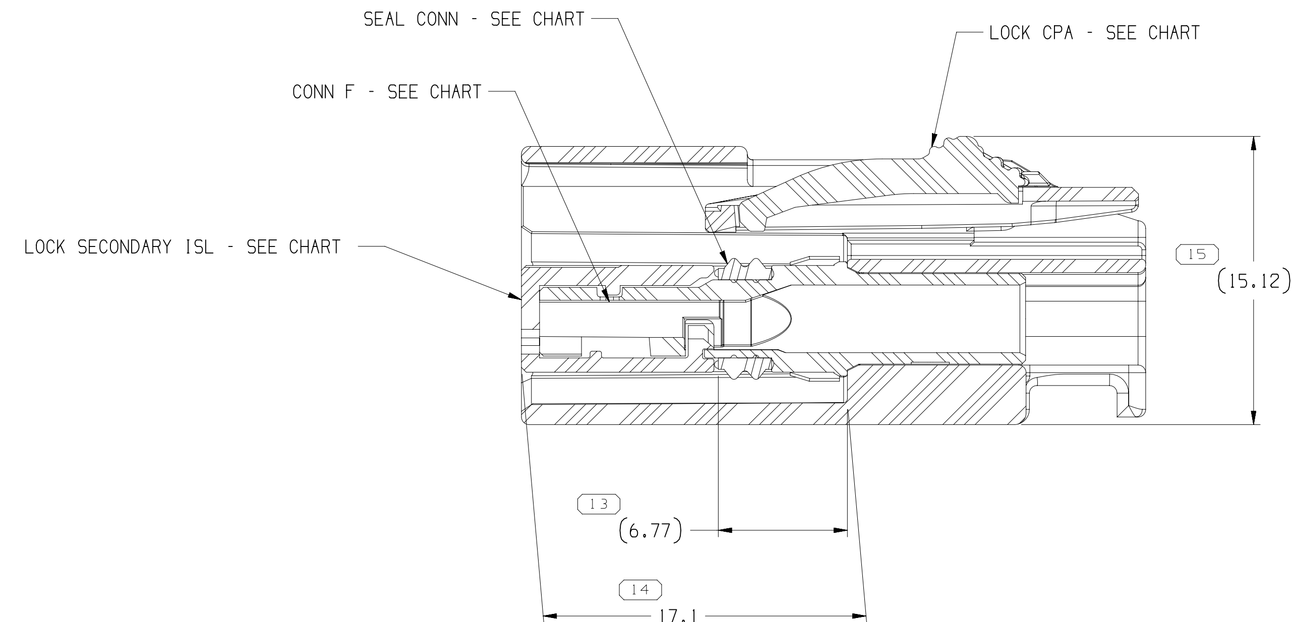
SECTION B-B
