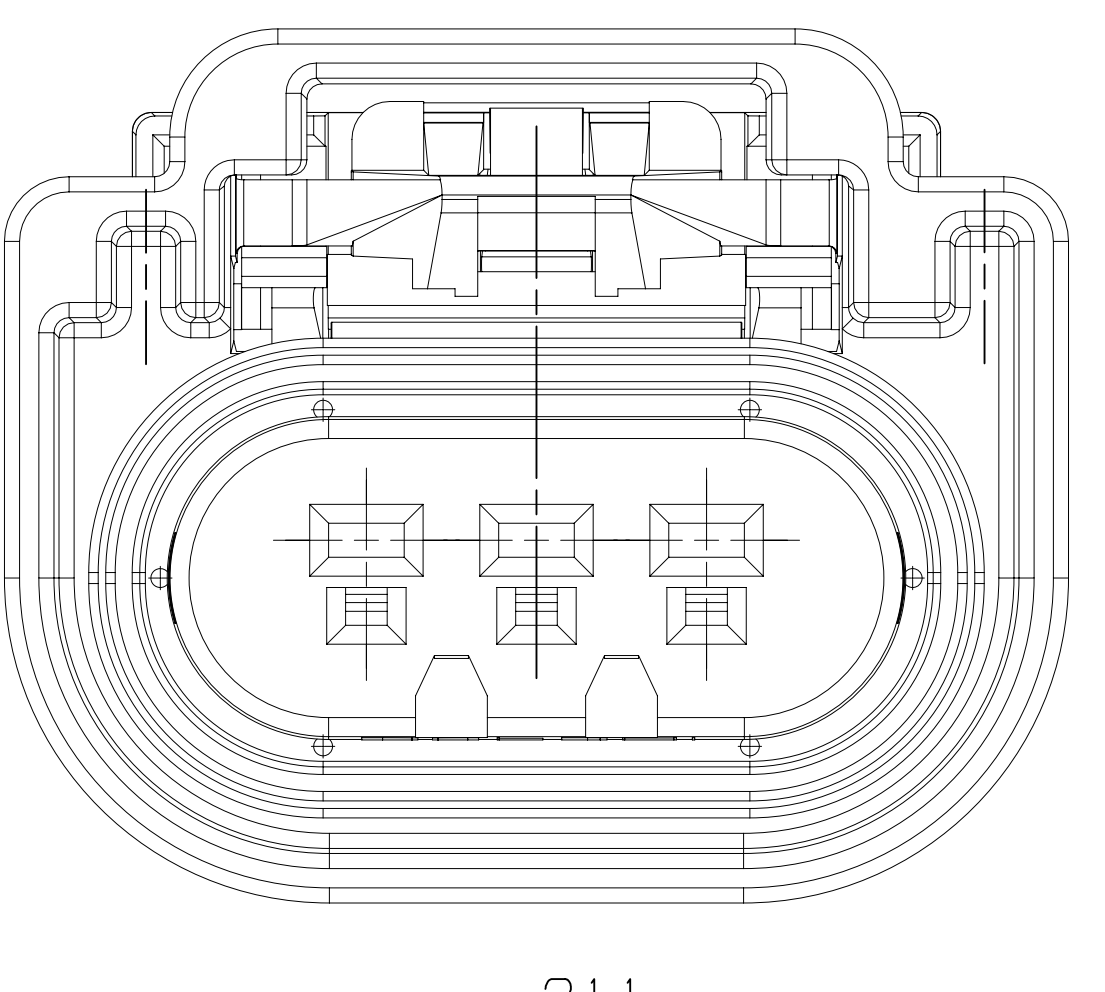
TYPE 211 SAME AS TYPE 201 EXCEPT AS SHOWN
