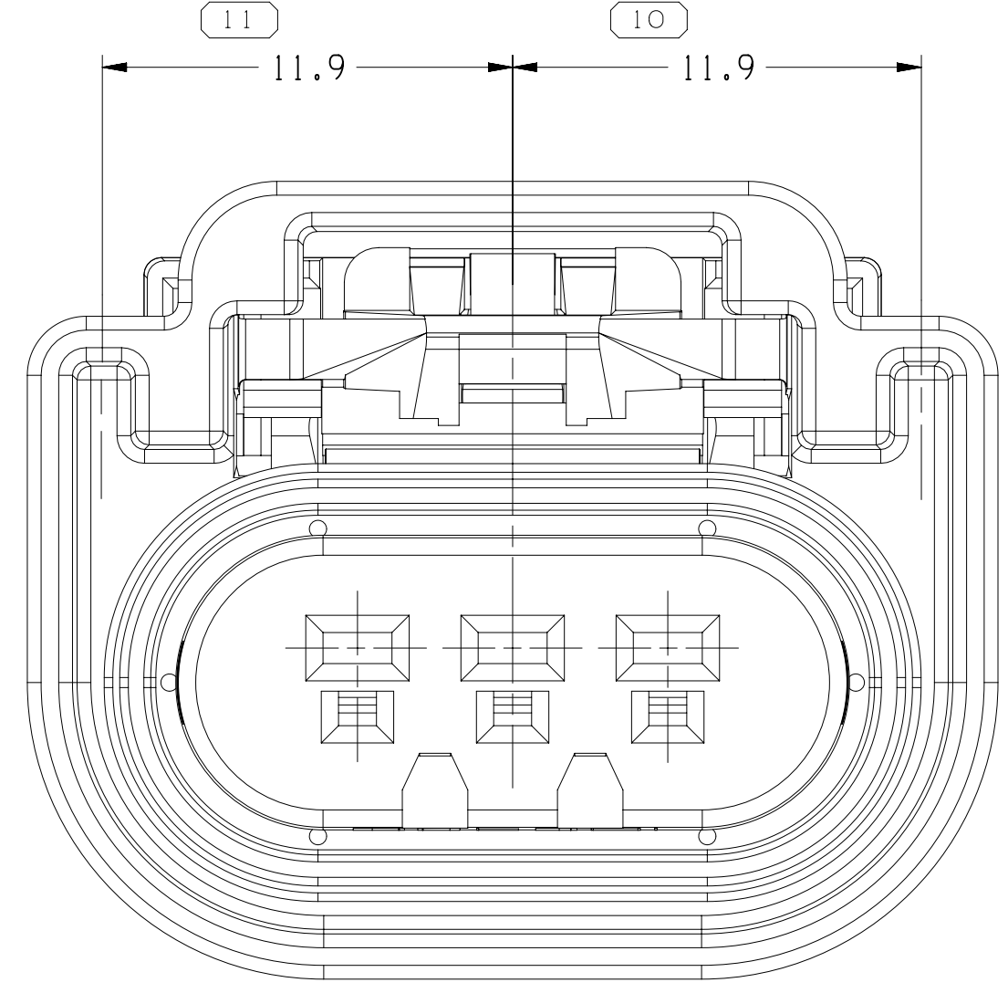
TYPE 203 SAME AS TYPE 202 EXCEPT AS SHOWN
