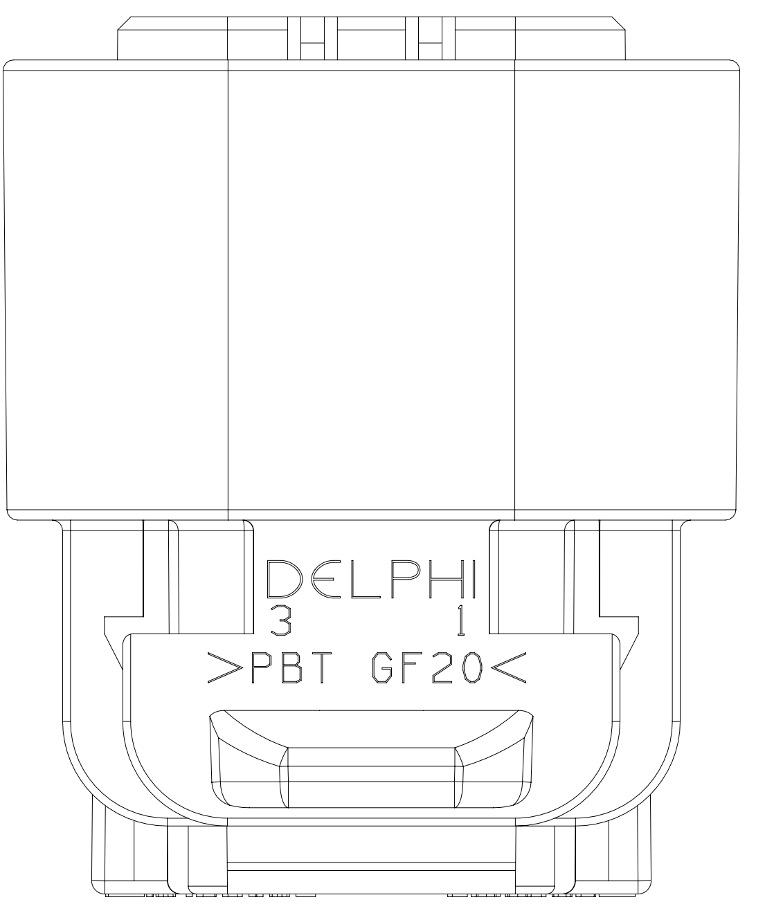
TYPE 202 SAME AS TYPE 201 EXCEPT MATL SPEC CALLOUT (SEE CHART 1) AND CAVITY IDENTIFICATION
