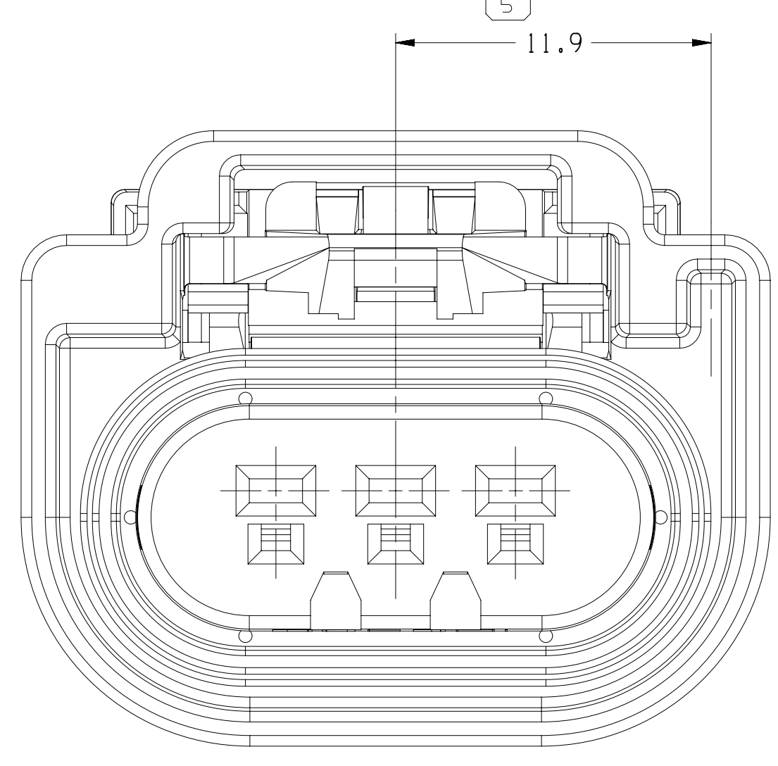
TYPE 206 SAME AS TYPE 202 EXCEPT AS SHOWN
