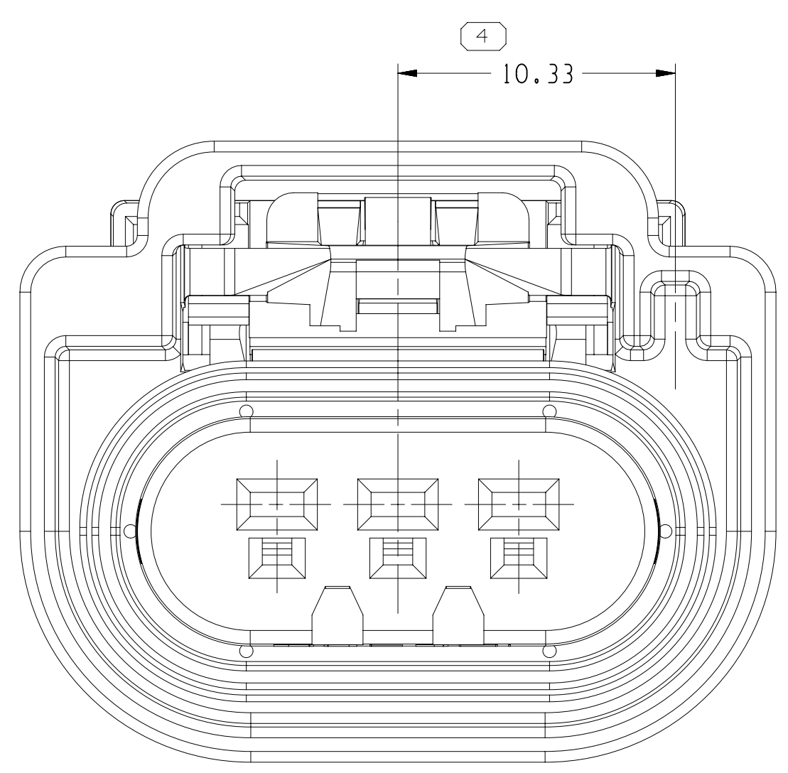
TYPE 207 SAME AS TYPE 202 EXCEPT AS SHOWN
