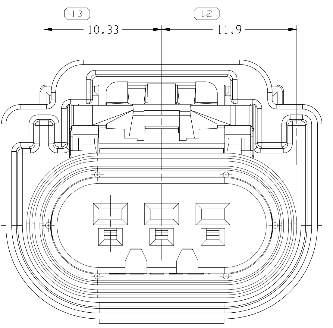
TYPE 202 SAME AS TYPE 201 EXCEPT MATL SPEC CALLOUT (SEE CHART 1) AND CAVITY IDENTIFICATION
