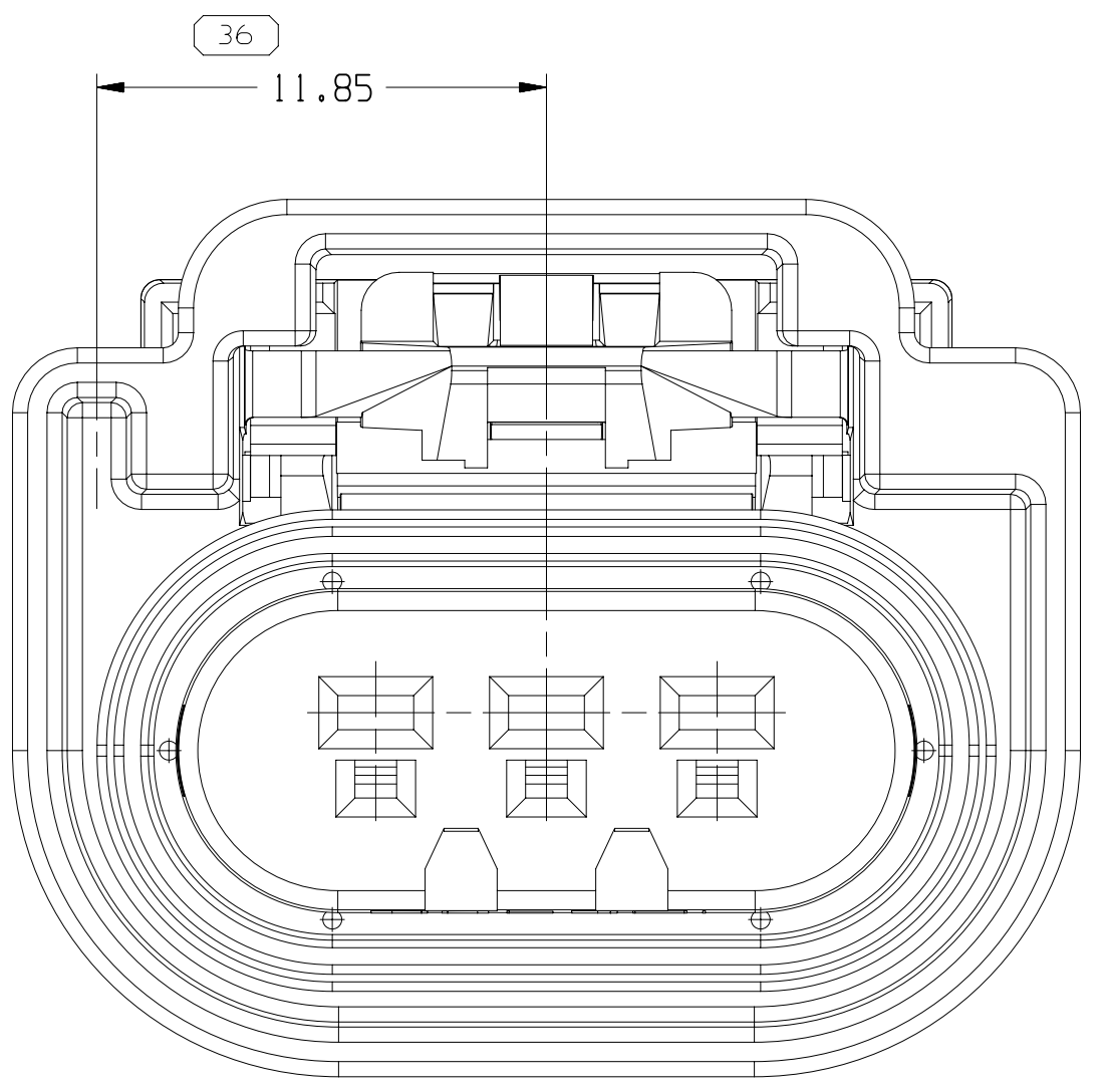
TYPE 212 SAME AS TYPE 202 EXCEPT AS SHOWN
