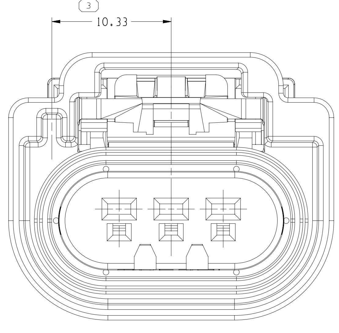
TYPE 208 SAME AS TYPE 202 EXCEPT AS SHOWN
