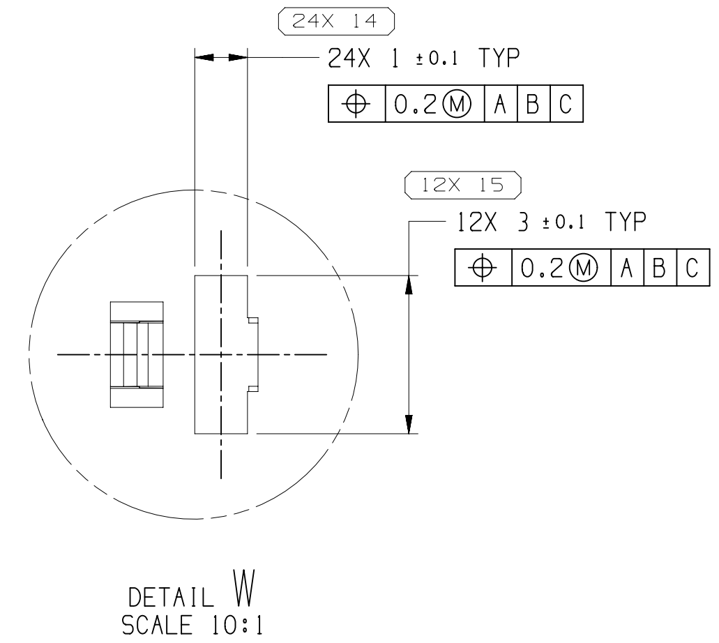
DETAIL W SCALE 10:1
