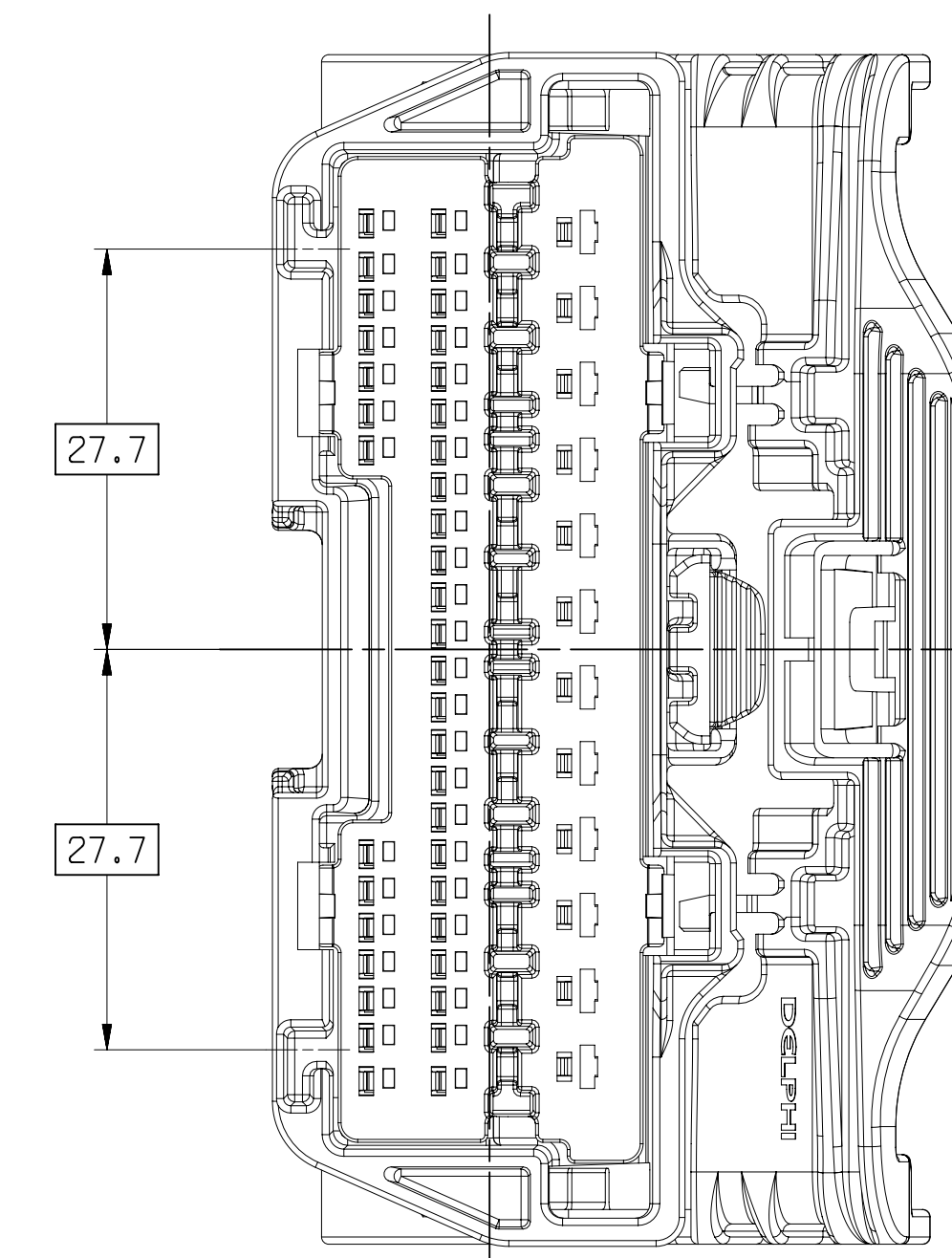
TYPE 102 SAME AS TYPE 101 EXCEPT AS SHOWN SCALE 2:1
