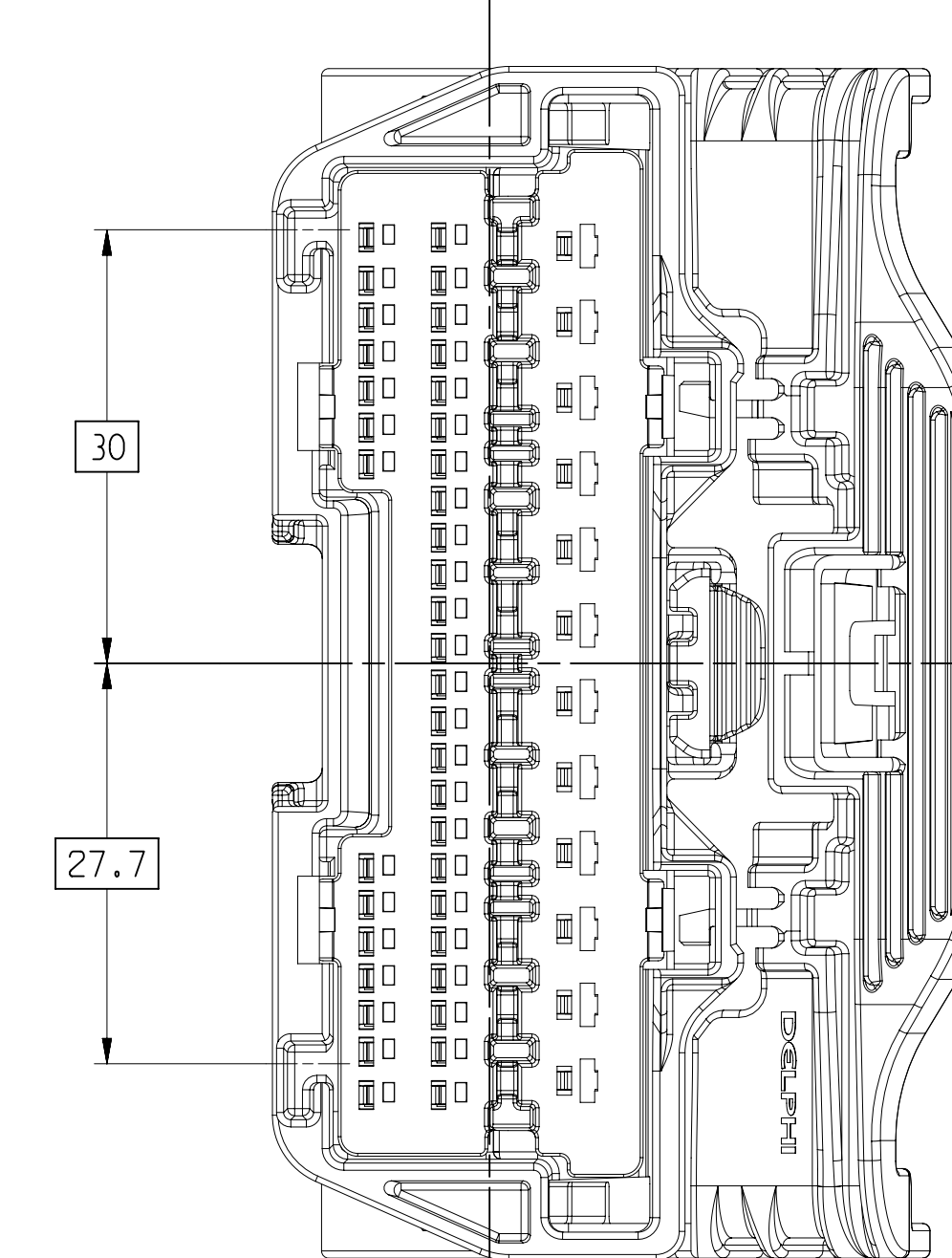
TYPE 103 SAME AS TYPE 101 EXCEPT AS SHOWN SCALE 2:1
