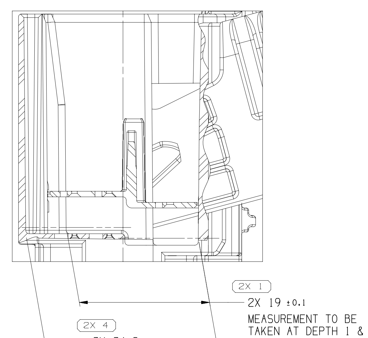
DETAIL V SCALE 3:1
