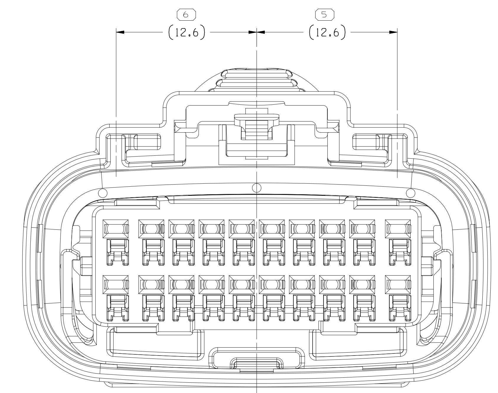
TYPE 104 SAME AS TYPE 101 EXCEPT AS SHOWN
