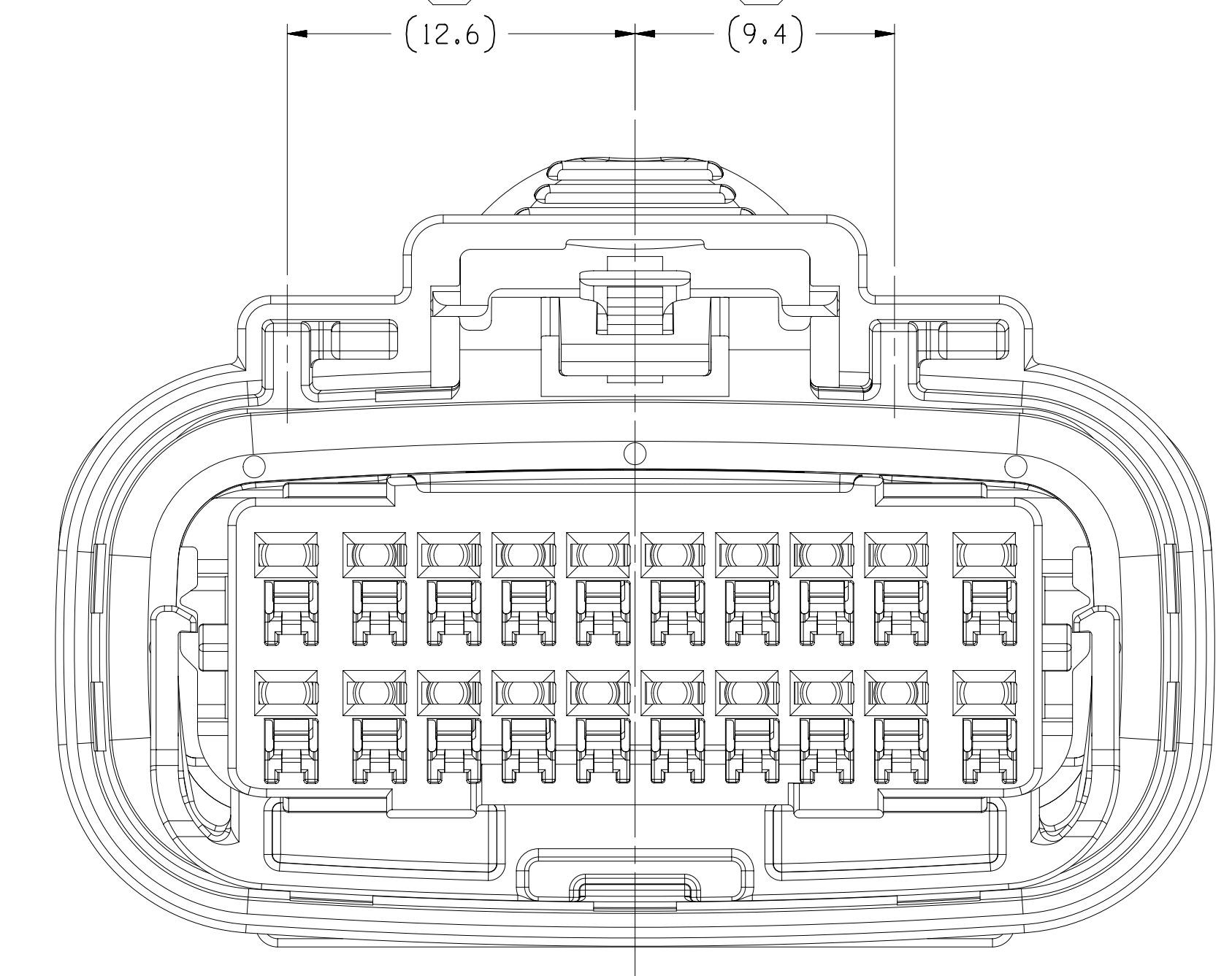
TYPE 102 SAME AS TYPE 101 EXCEPT AS SHOWN
