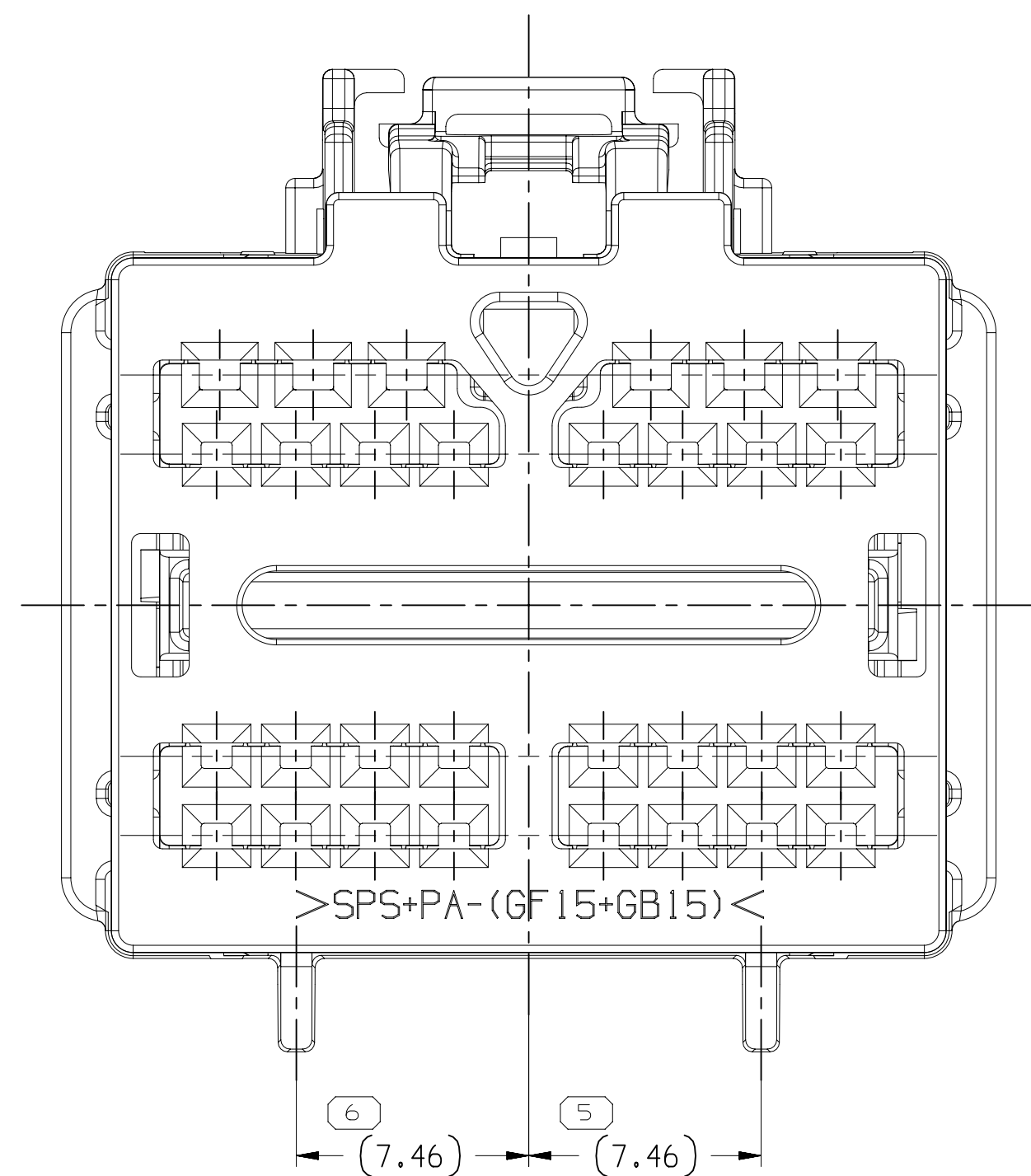
TYPE 104 SAME AS TYPE 101 EXCEPT AS SHOWN
