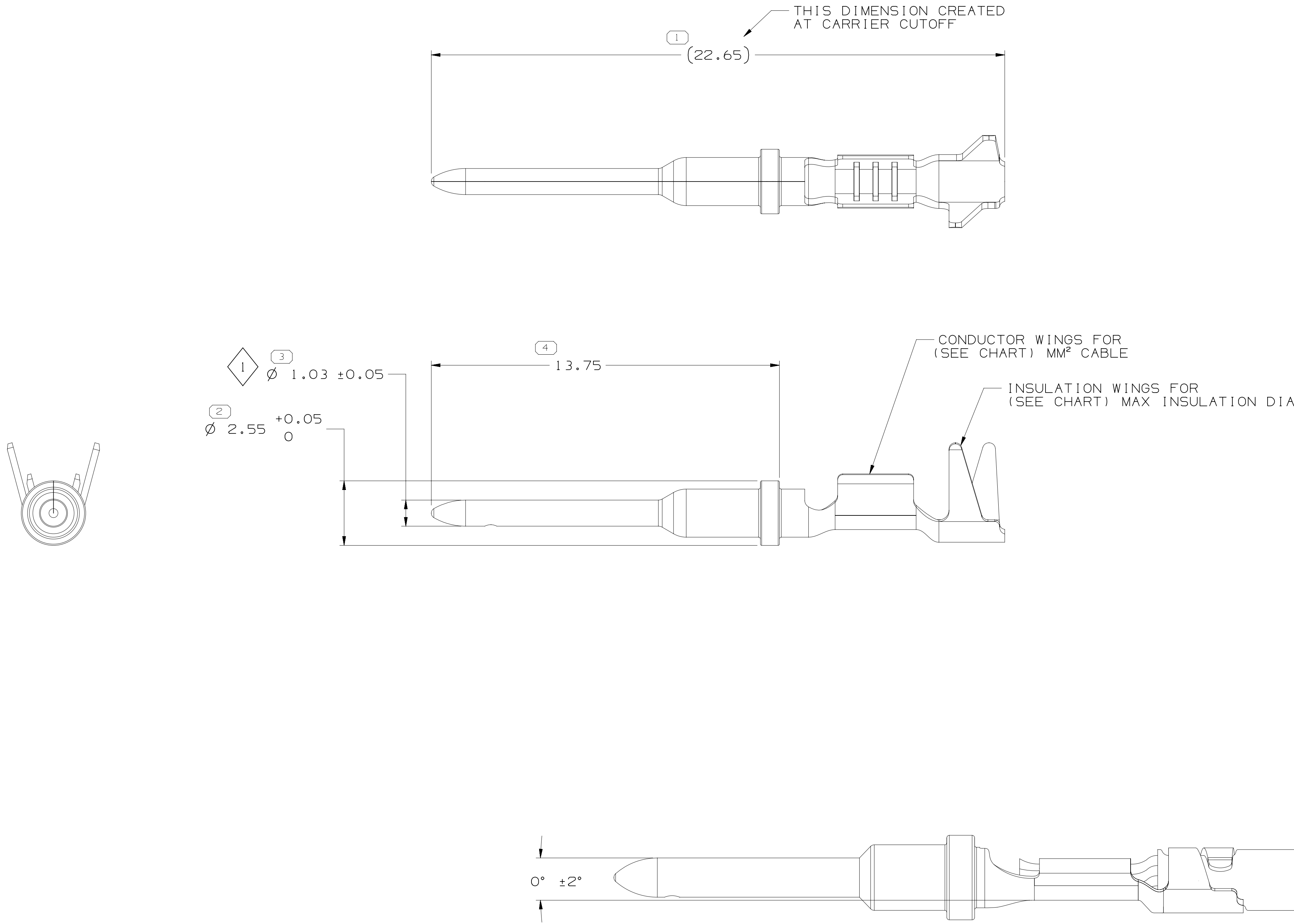
CRIMPED TERMINAL AND CABLE ALIGNMENT
