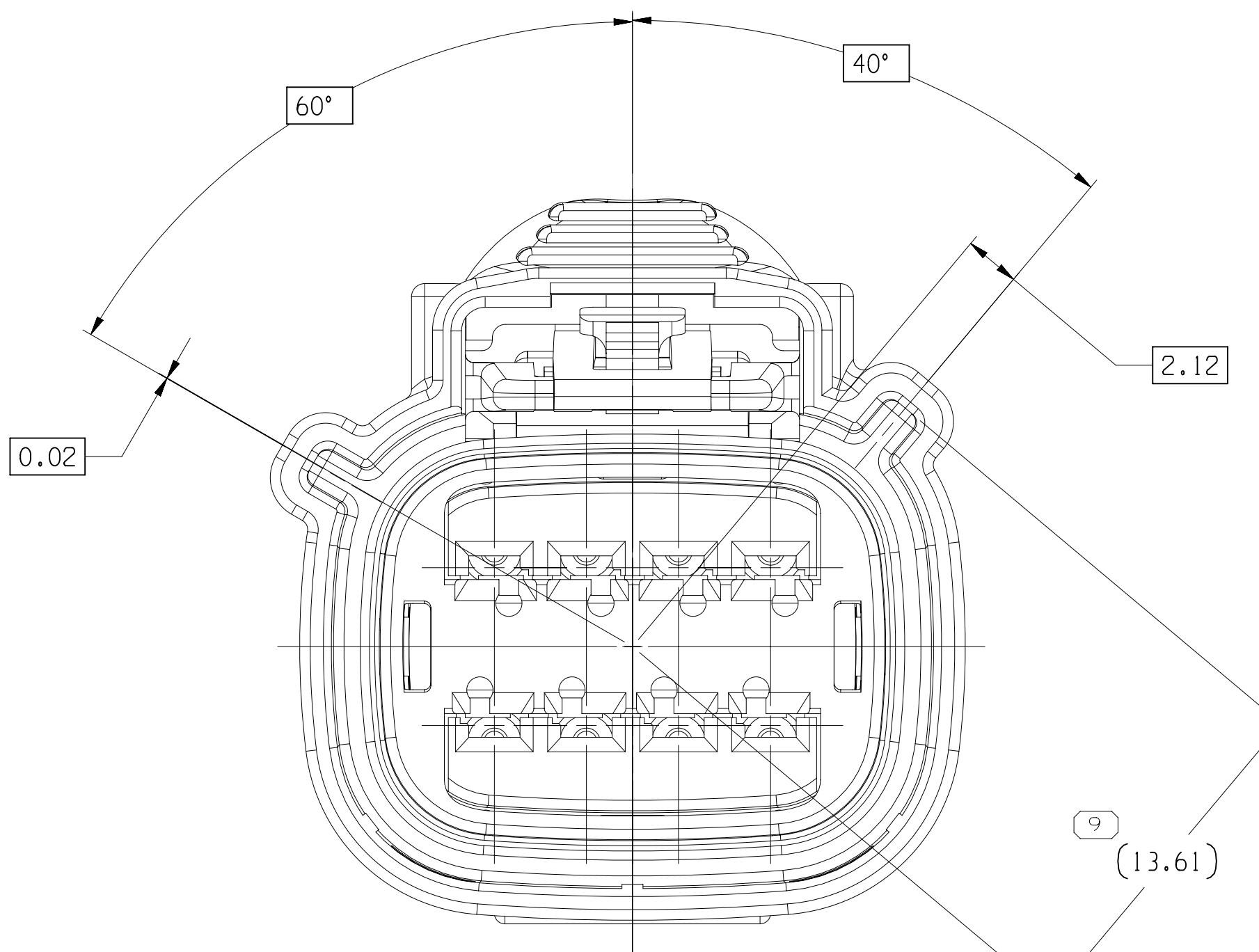
TYPE 106 SAME AS TYPE 101 EXCEPT AS SHOWN
