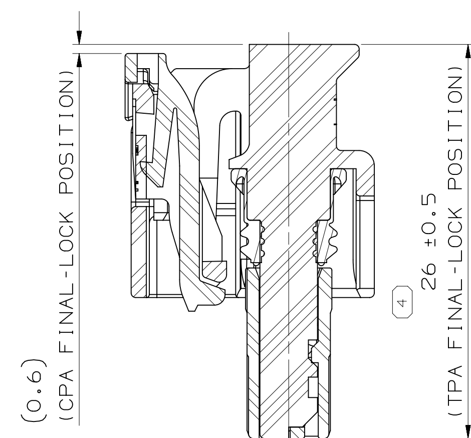
SECTION B-B CPA & TPA IN FINAL POSITION
