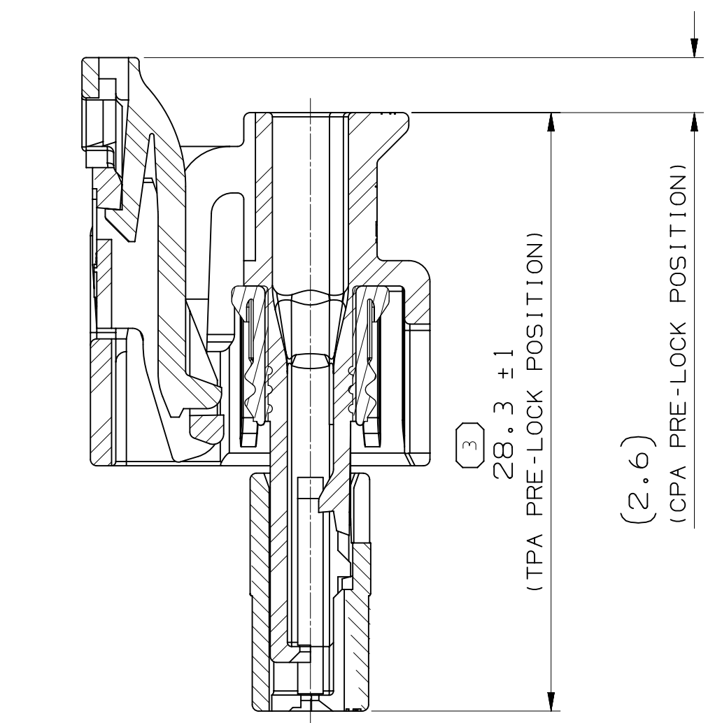
SECTION A - A CPA & TPA IN PRE-LOCK POSITION
