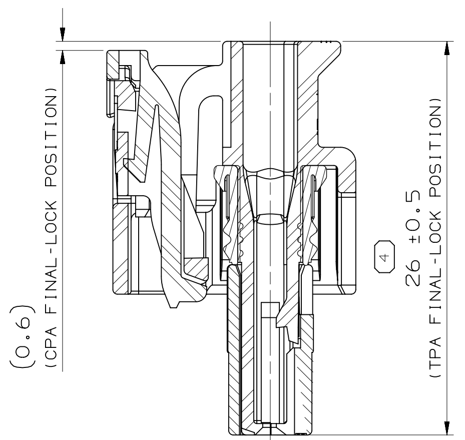
SECTION B - B CPA & TPA IN FINAL POSITION
