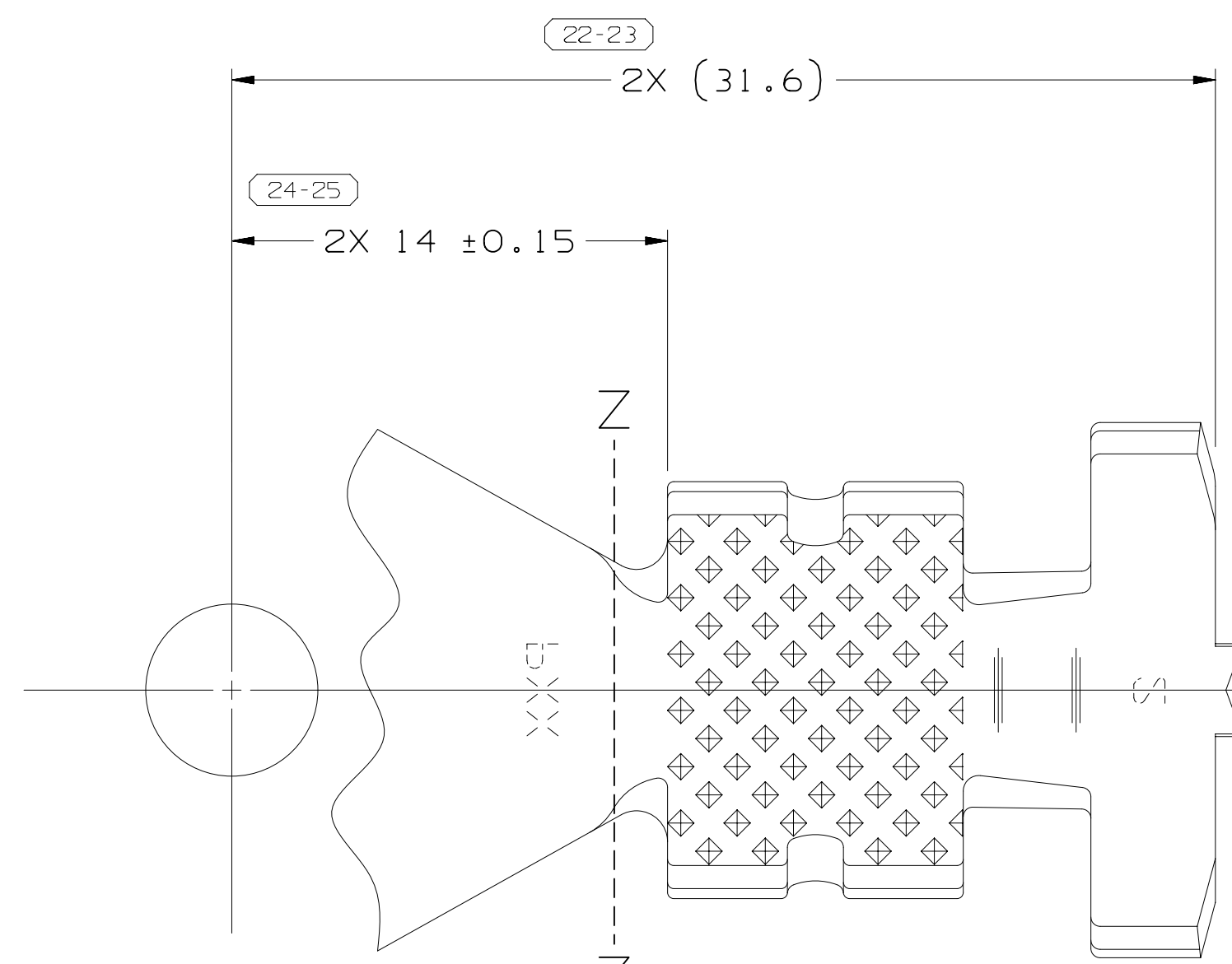
(32 MM²) TYPE 821/822 SAME AS TYPE 801/802 EXCEPT AS SHOWN
