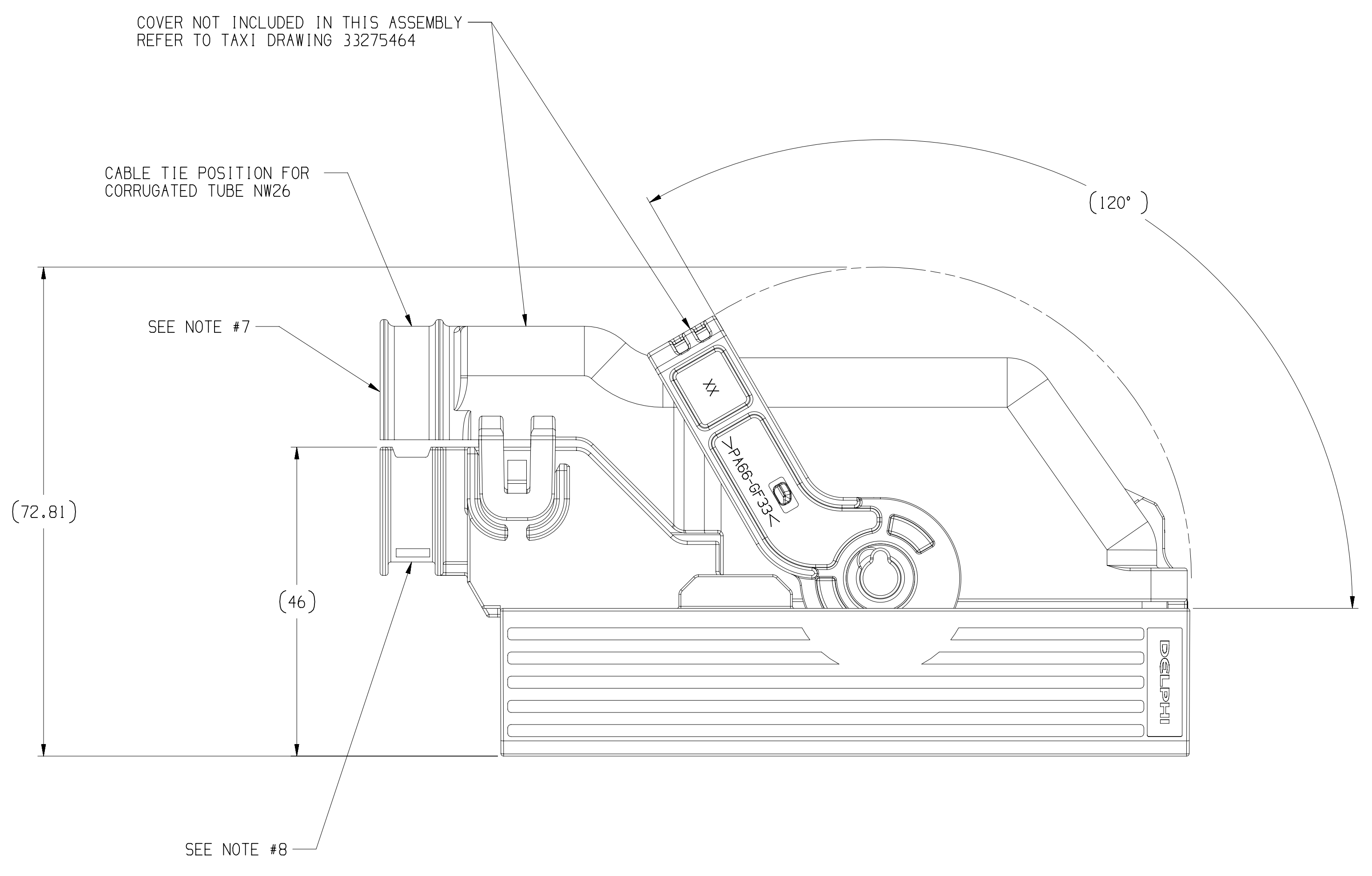
CONNECTOR IN PRE-LOCKED POSITION INCL. COVER
