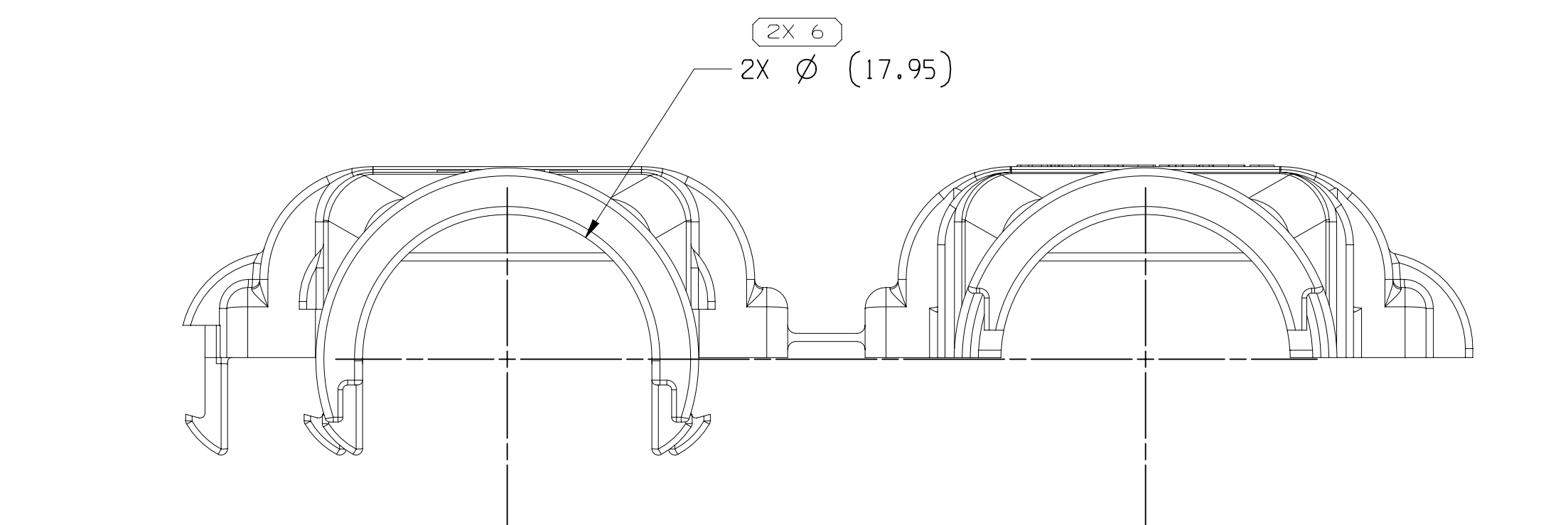
33321084 - NO CONDUIT SAME AS TYPE 13mm CONDUIT EXCEPT AS SHOWN
