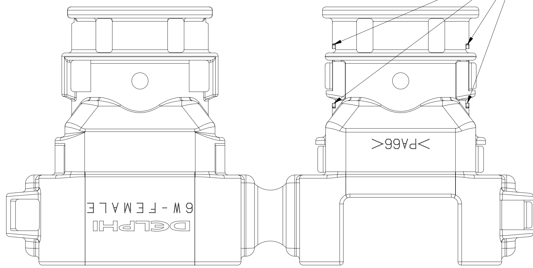
OPTIONAL CONSTRUCTION VIEW
