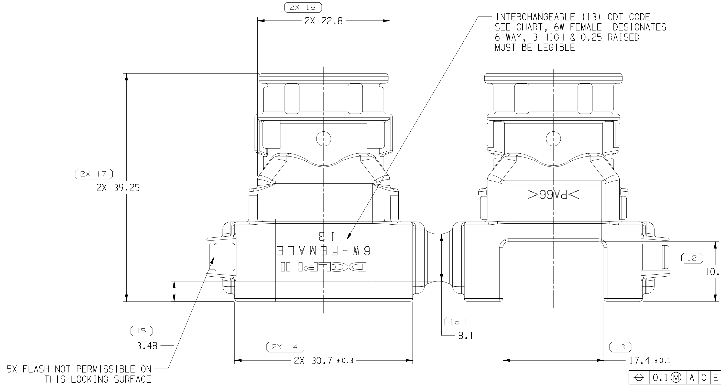
5X FLASH NOT PERMISSIBLE ON THIS LOCKING SURFACE
