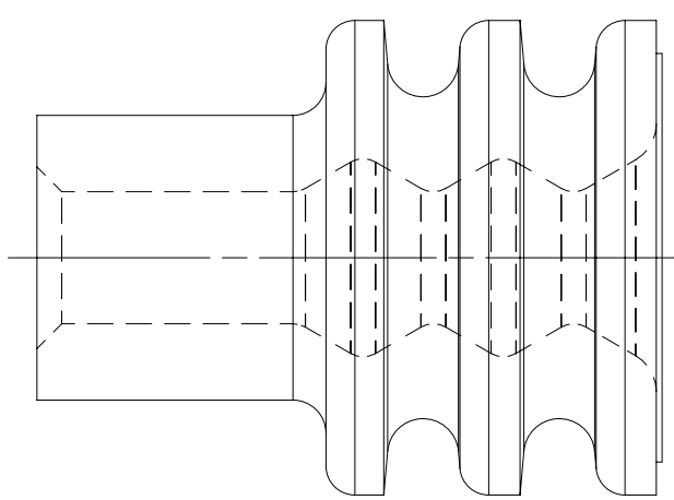
OPTIONAL CONSTRUCTION 1 (ANTI-STICK RING)
