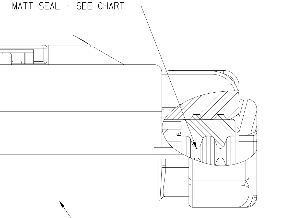
TYPE A - SEALED ASSEMBLY
