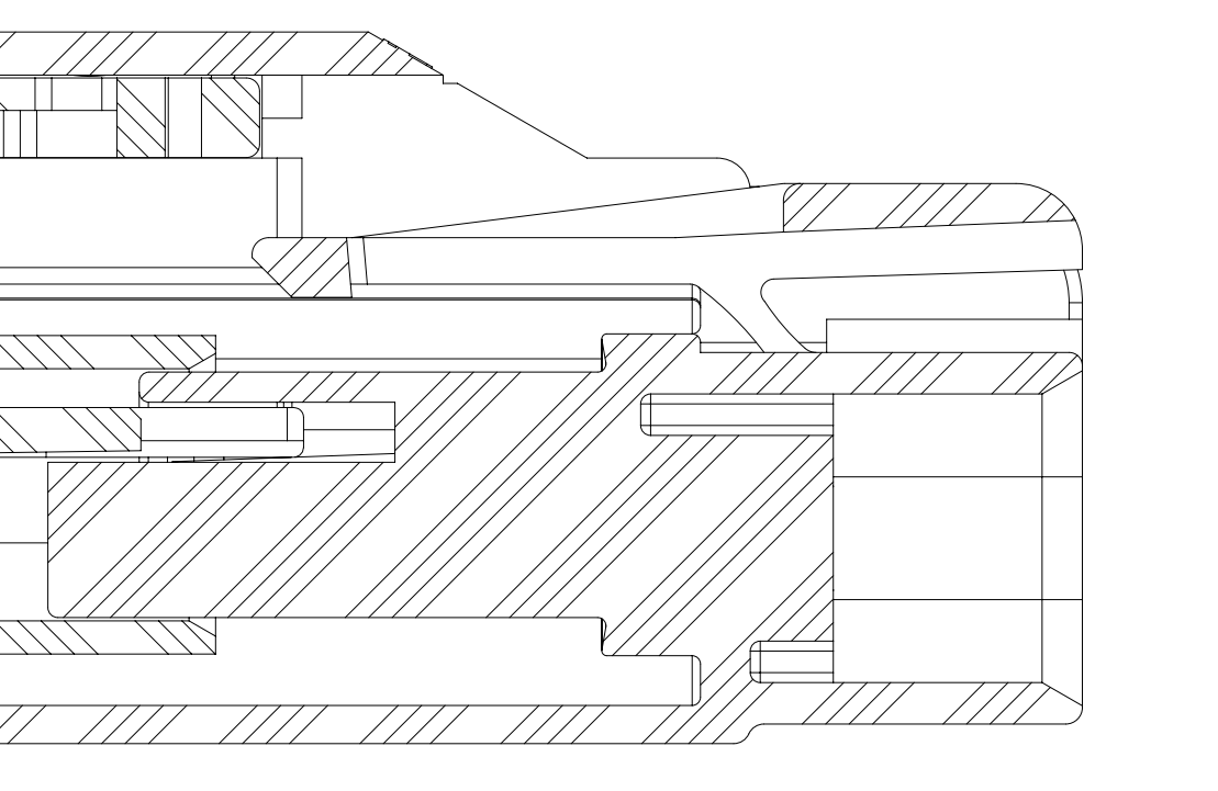
SECTION B-B
