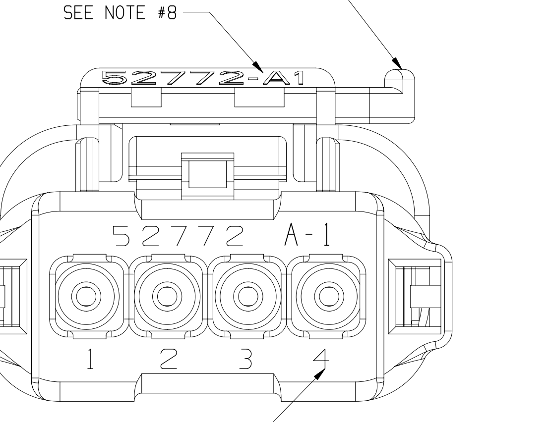
TYPE A - UNSEALED ASSEMBLY
