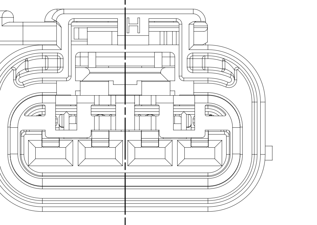
AUXILIARY FRONT VIEW TYPE A - UNSEALED ASSEMBLY
