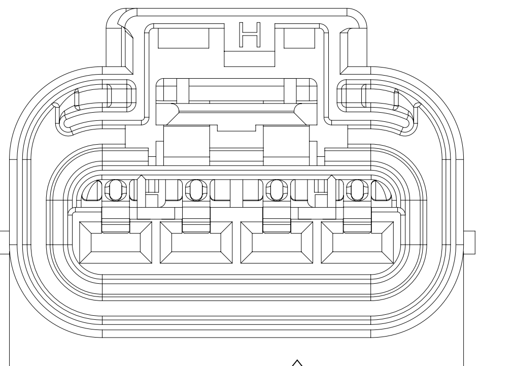
AUXILIARY VIEW TYPE A - CONNECTOR VIEW FOR REFERENCE ONLY (SEE DIM "A" ON TAXI PART NO 3351932/C17001-CUST)
