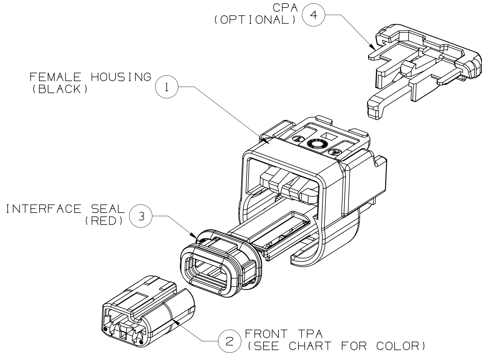
EXPLODED VIEW
