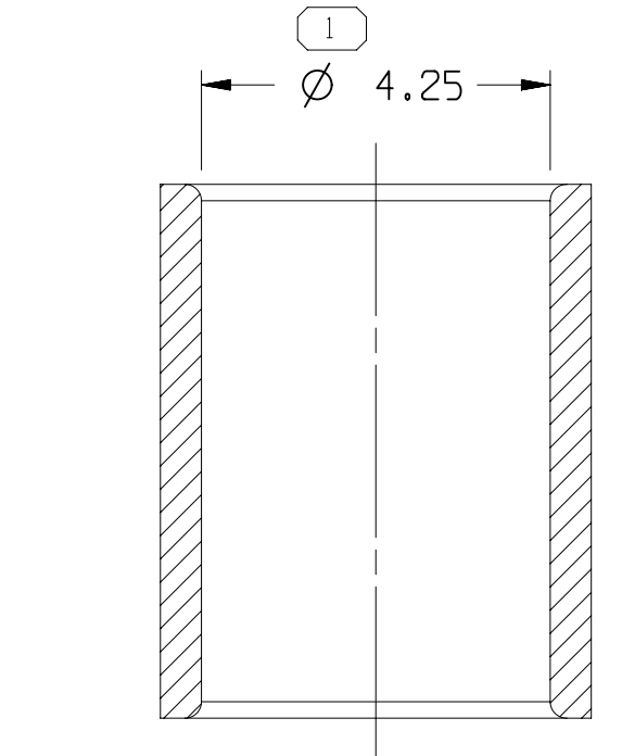
SECTION C - C TYPE 103 SAME AS TYPE 101 EXCEPT AS SHOWN
