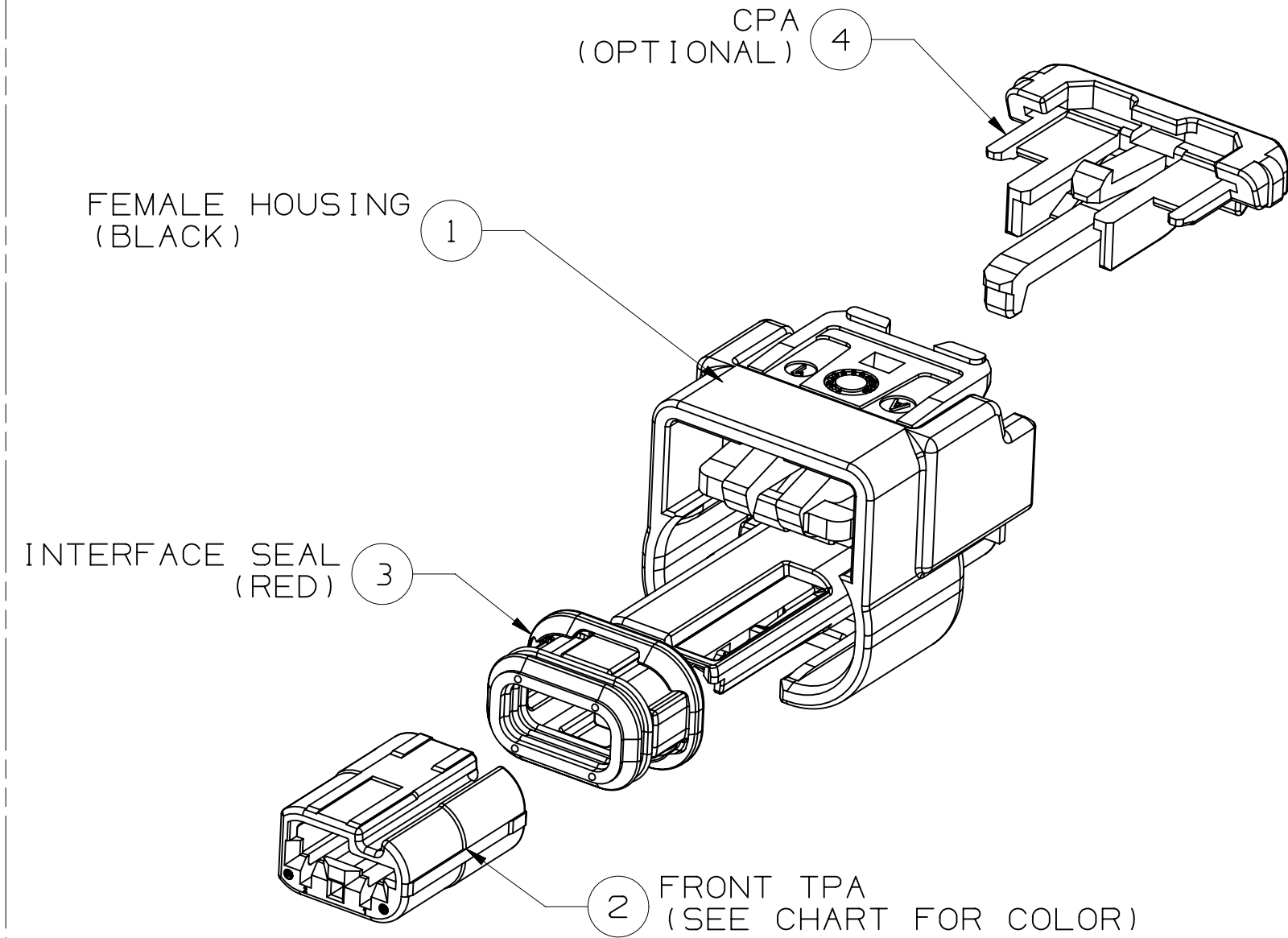
EXPLODED VIEW
