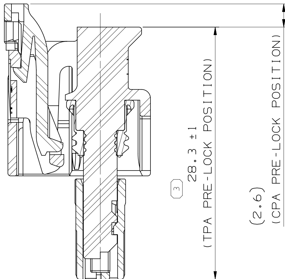
SECTION A-A CPA & TPA IN PRE-LOCK POSITION
