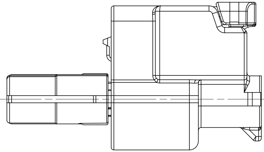
SECTION A-A CPA & TPA IN PRE-LOCK POSITION
