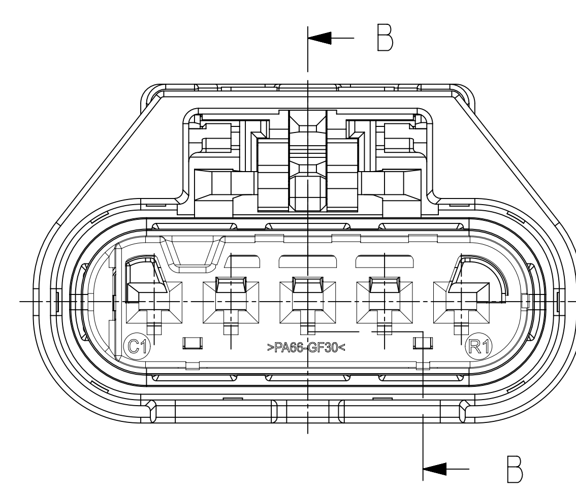
C.P.A & T.P.A IN FINAL LOCK POSITION
