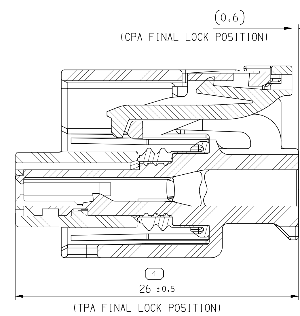
SECTION B-B
