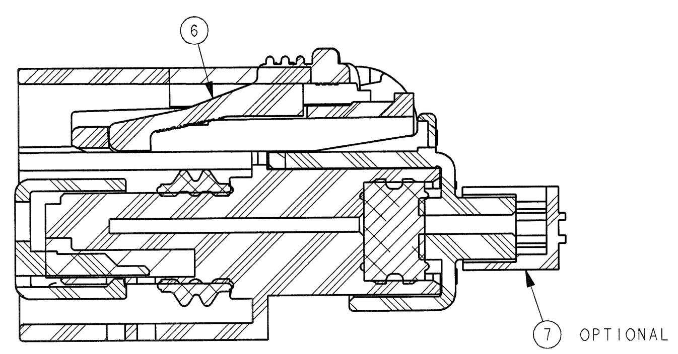
SECTION A-A TPA SHOWN IN PRE-LOADED POSITION
