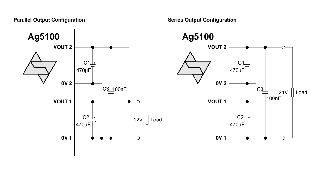
Figure 6: Output Configurations
