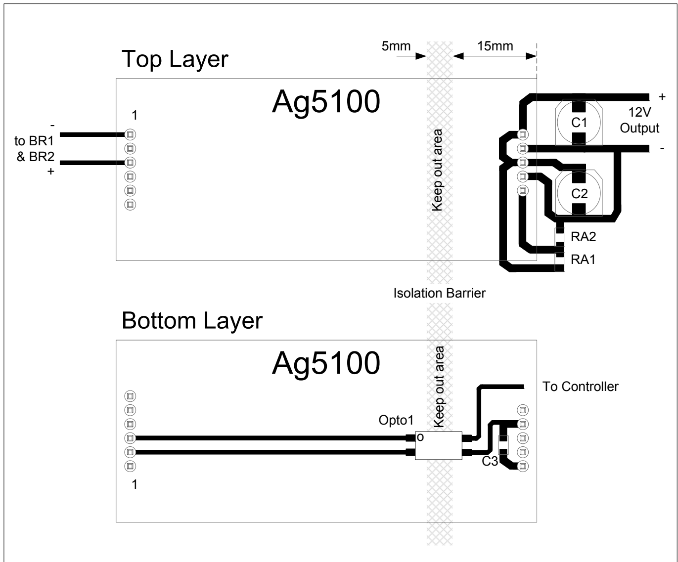
Figure 10: Typical Layout
