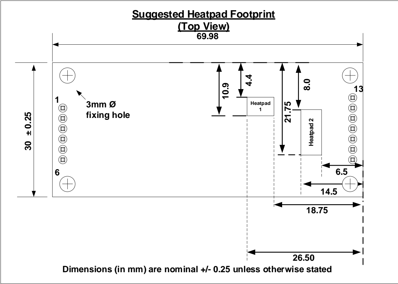
Figure 12: Suggested Heatpad Footprint
