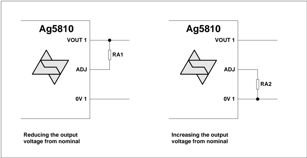
Figure 6: Output Adjustment
