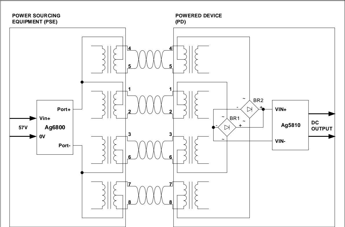
Figure 8b – Typical Application Diagram for Ag6800 using 1000BASE-T
