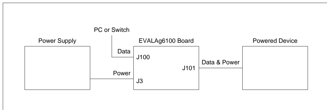
Figure 4: Basic set-up
