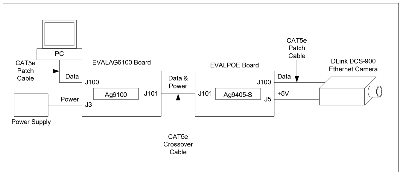
Figure 5: Example set-up
