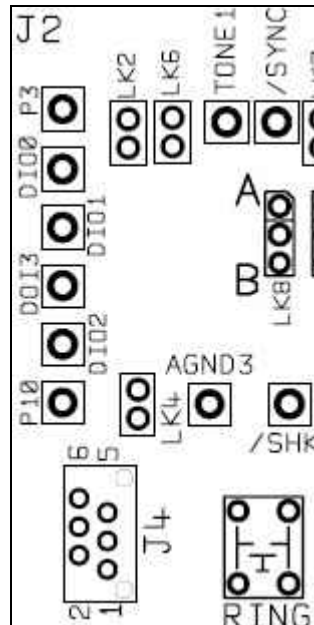
Figure 12: Other Links
