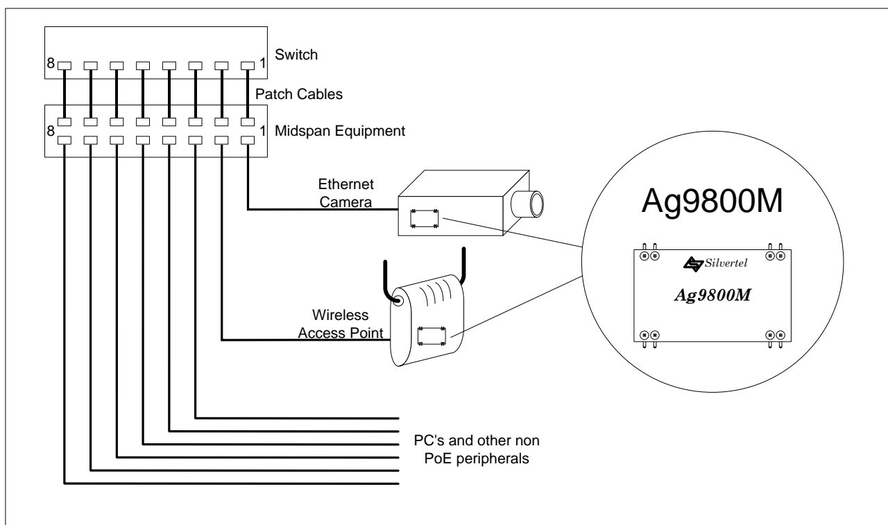
Figure 7: Typical Application
