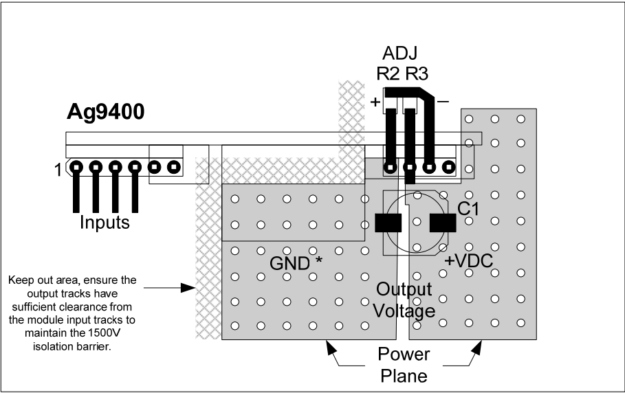
Figure 8: Power Plane Heatsink for Ag9400
