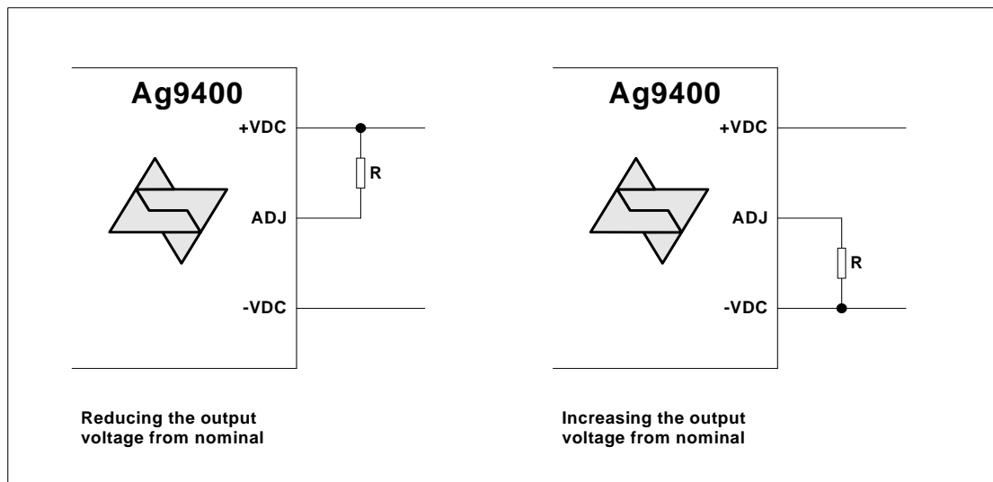
Figure 4: Output Adjustment
