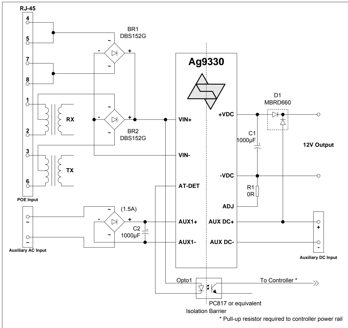
Figure 7: Typical PoE and Auxiliary Input Connection Diagram
