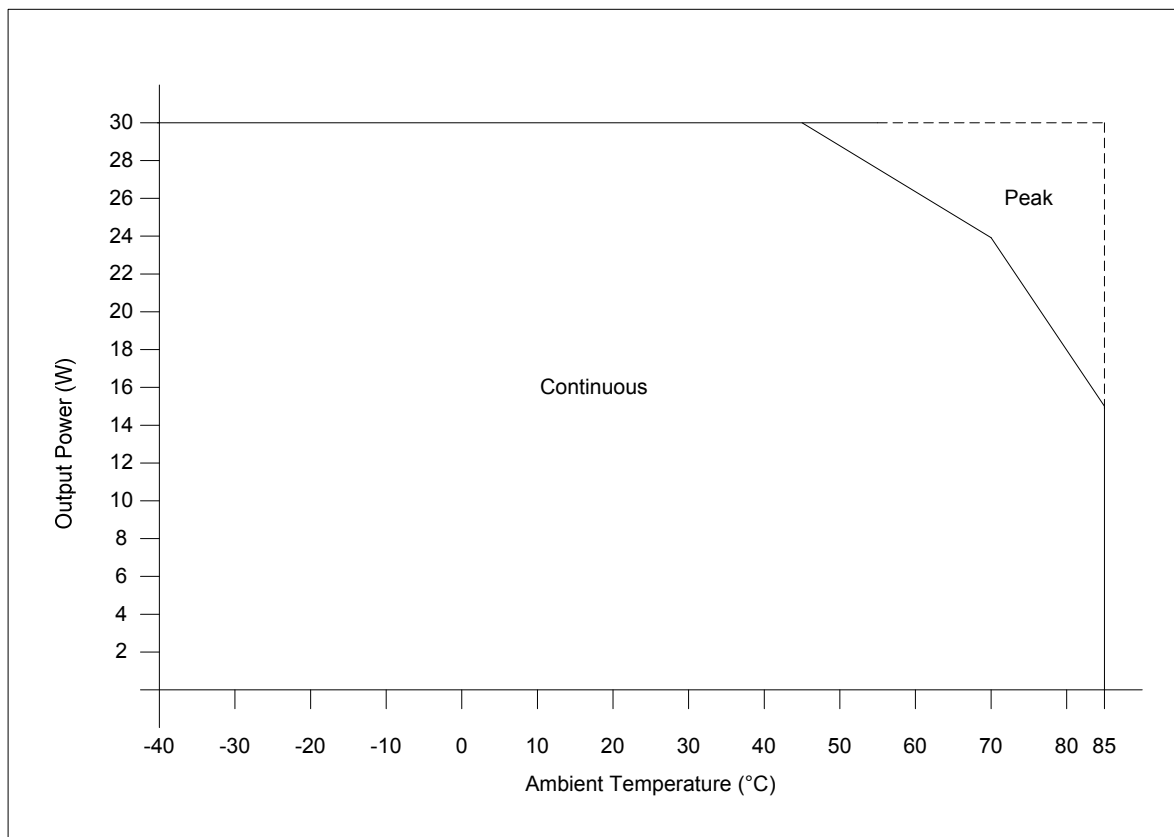
Figure 10: Ag9330 Operating Profile
