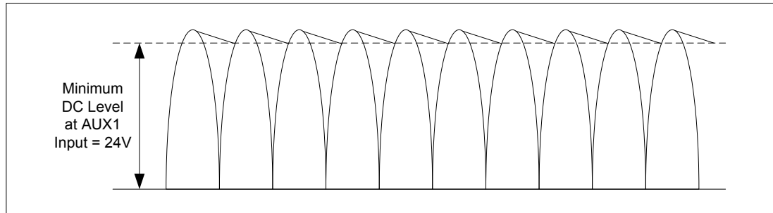
Figure 8: Minimum DC voltage at the AUX1 input
