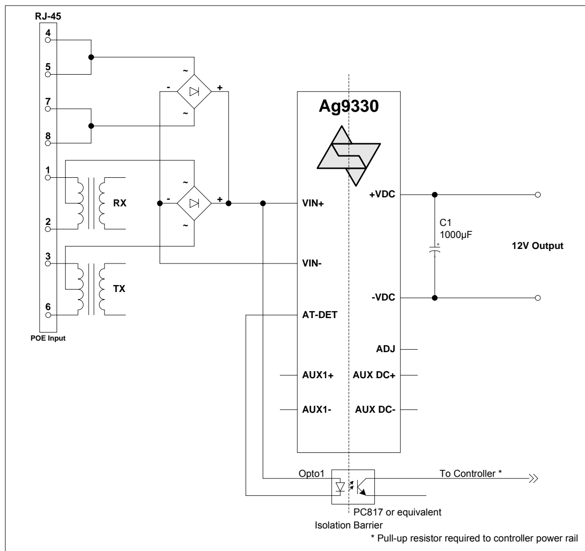
Figure 6: Typical PoE Only Connection Diagram
