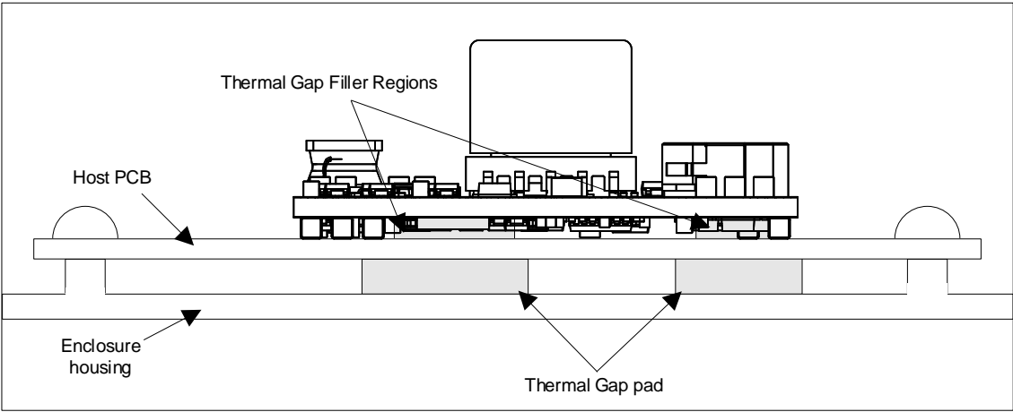
Figure 9: Additional Heatsinking
