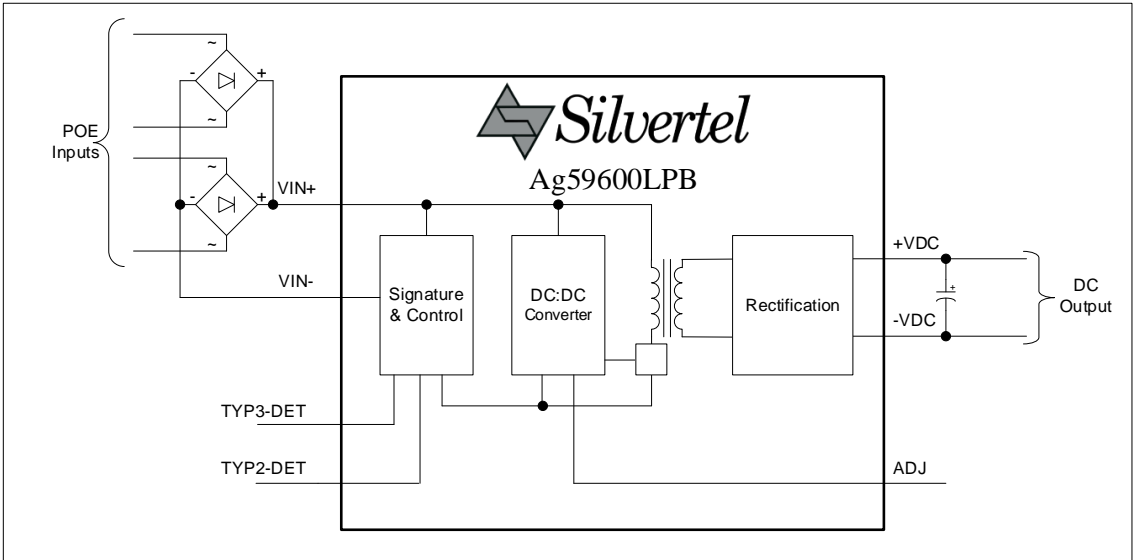
Figure 1: Block Diagram
