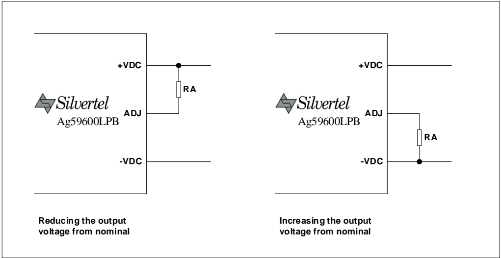
Figure 5: Output Voltage Adjustment
