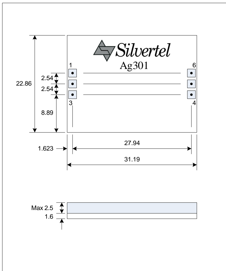
Figure 11: Package Dimensions
