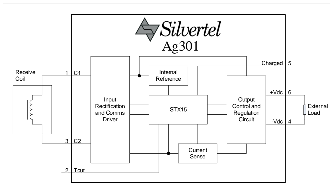
Figure 1: Block Diagram
