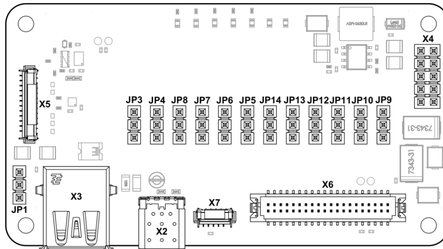
Fig. 2. Verdin iMX8M Plus Mezzanine (top side, top view)
