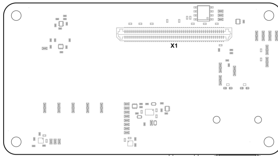
Fig. 3. Verdin iMX8M Plus Mezzanine (bottom side, bottom view)
