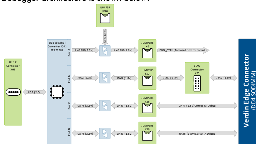
Figure 11: USB Debugger architecture
