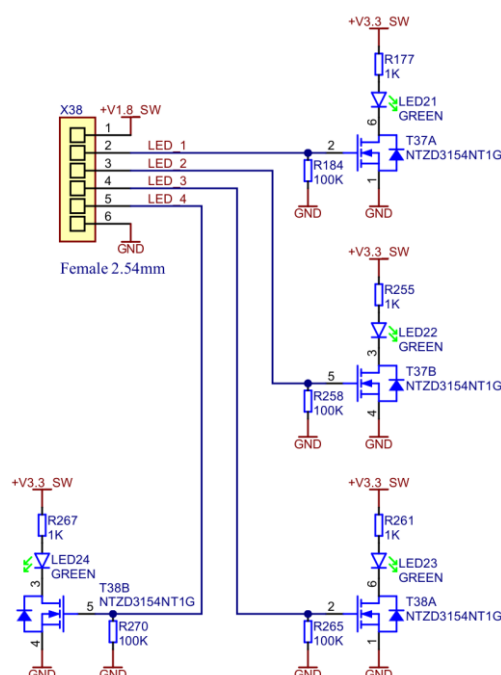
Figure 9: General-purpose LEDs' schematic
