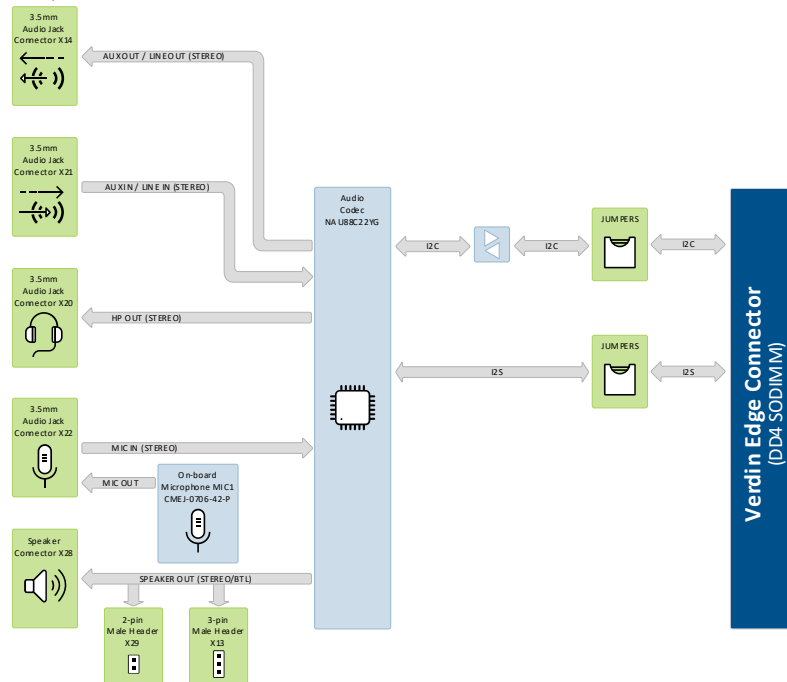
Figure 7: Analog Audio architecture
