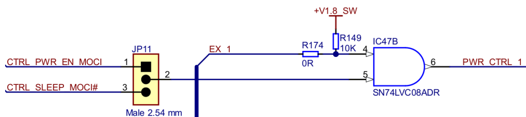
Figure 4: Part of the power gating schematic
