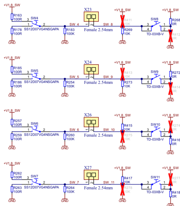
Figure 8: General-purpose switches' schematic
