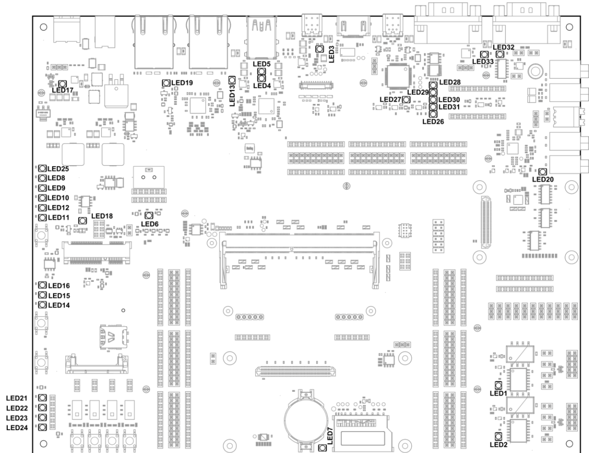
Figure 5: Indicator LEDs
