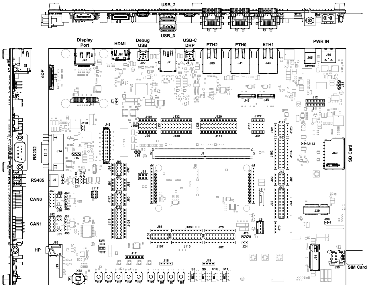
Figure 2: SMARC Development Board connectors and controls
