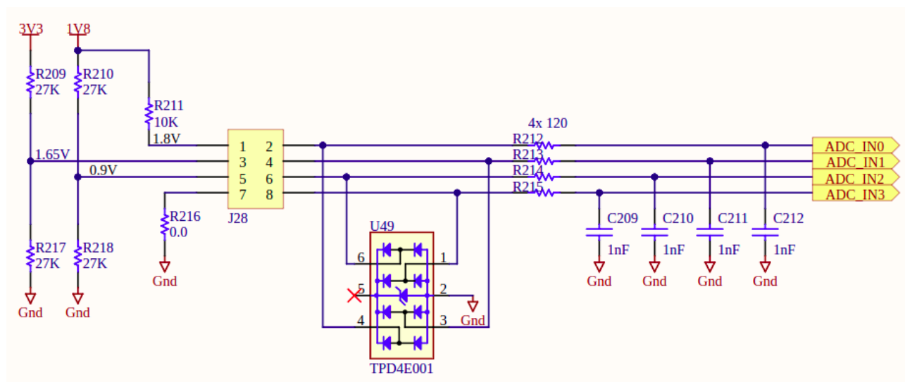
Figure 4: ADC Connector (J28 and J29)
