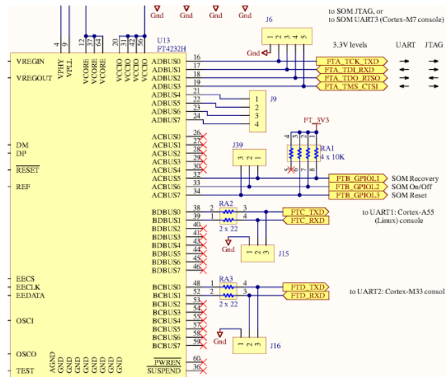
Figure 24: FTDI
