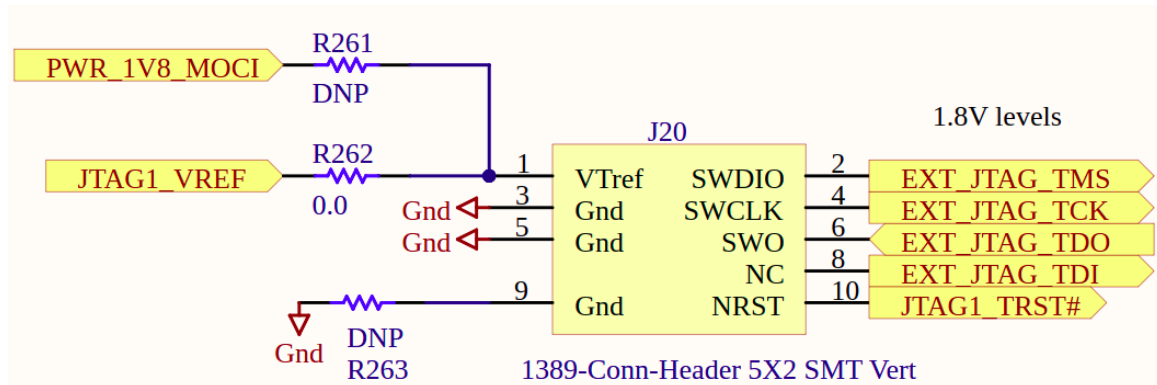
Figure 28: JTAG Connector (J20)
