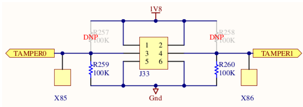
Figure 42: Tamper (J33)
