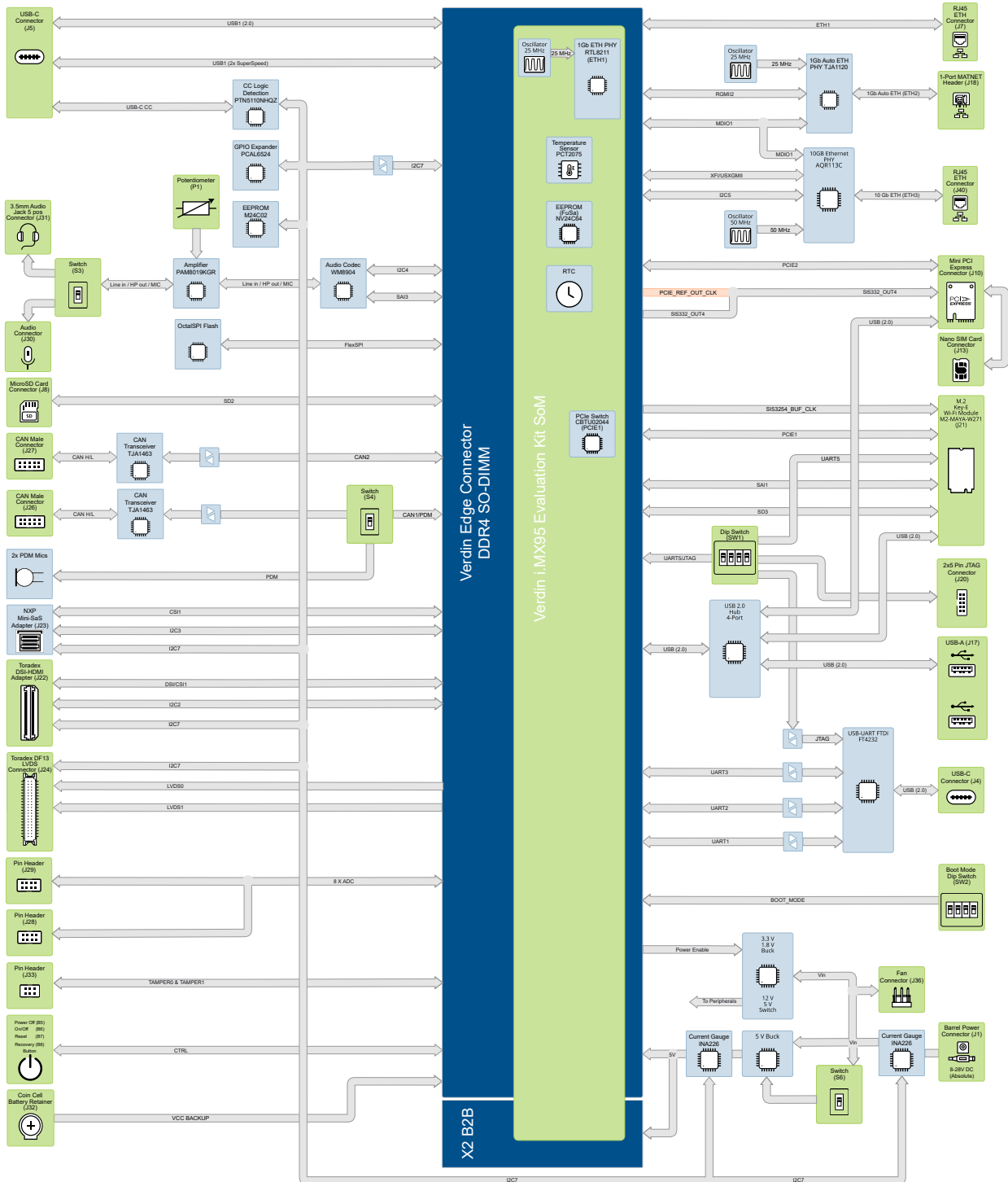
Figure 1: i.MX 95 Verdin Evaluation Kit Hardware Architecture
