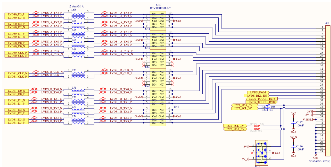
Figure 18: LVDS Connector (J24)
