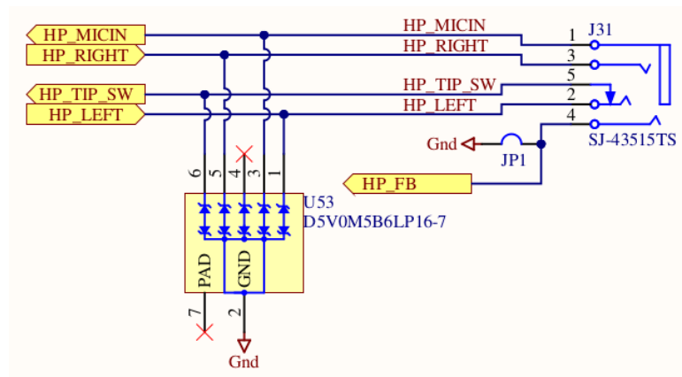
Figure 6: Audio Connector (J31)
