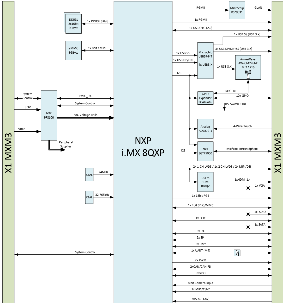
Figure 2 Apalis iMX8QXP 2GB WB IT Block Diagram
