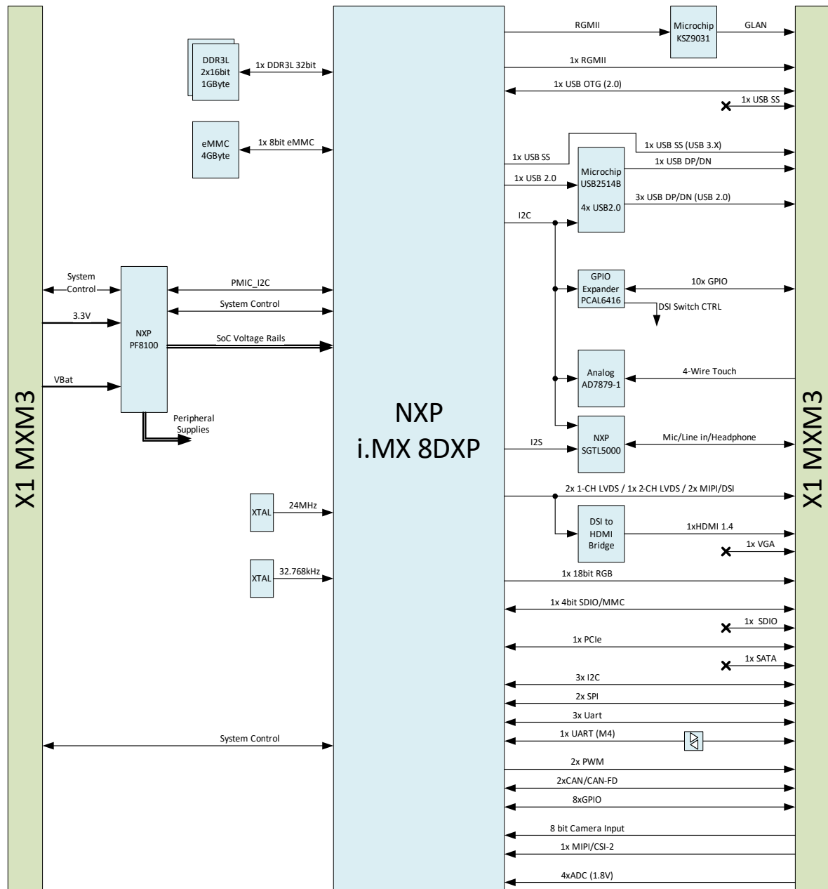
Figure 4 Apalis iMX8DXP 1GB Block Diagram
