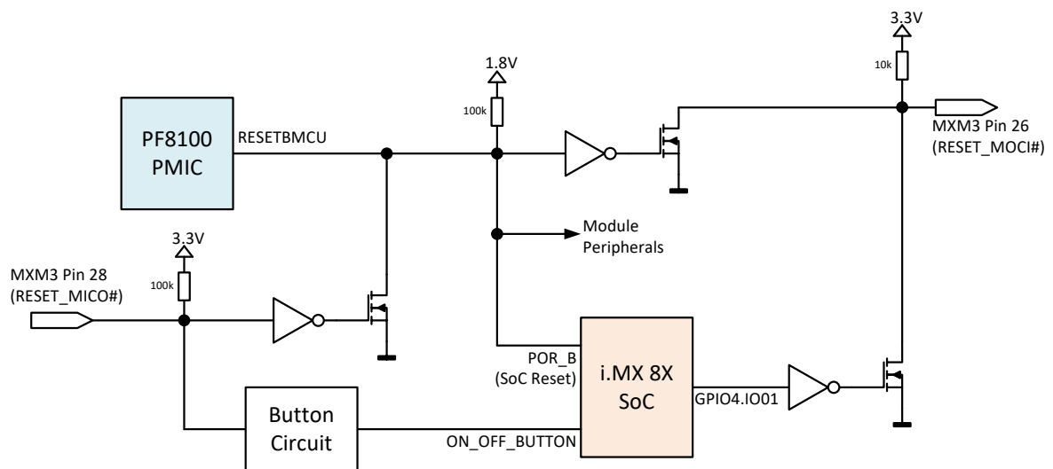
Figure 7 RESET_MOCI# circuit
