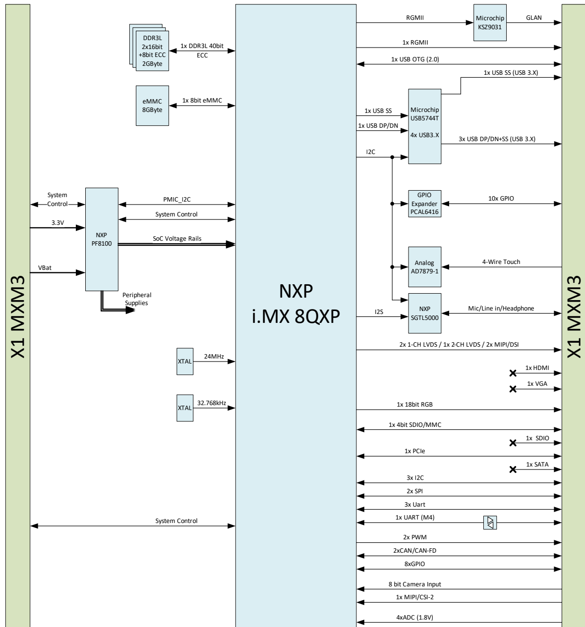
Figure 3 Apalis iMX8QXP 2GB ECC IT Block Diagram
