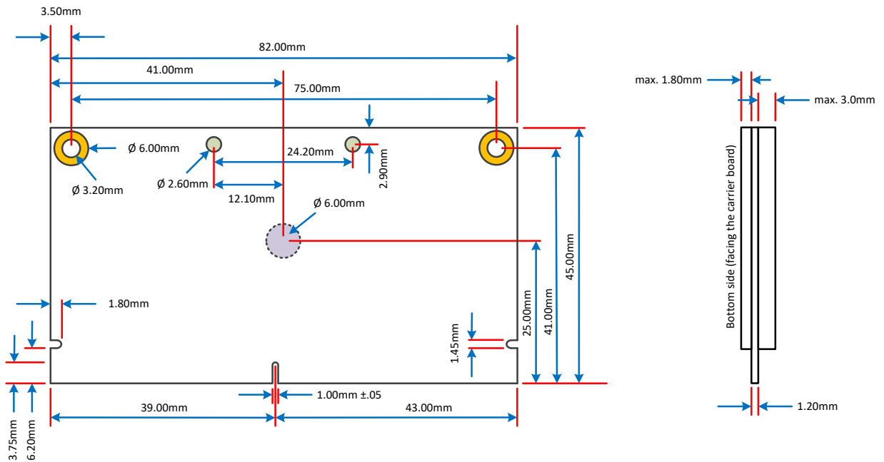
Figure 17 Mechanical dimensions of the Apalis module (top view) Tolerance for all measures: \pm 0.1\text{mm}
