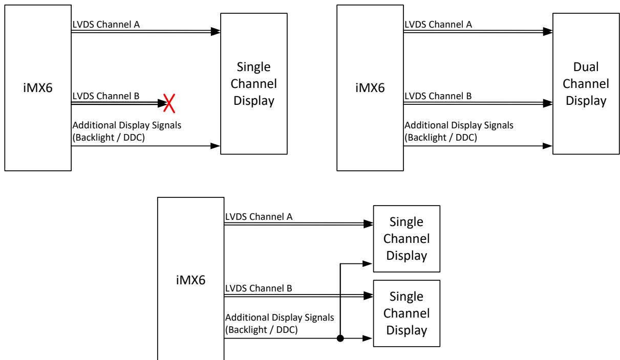
Figure 10: Available LVDS Display configurations
