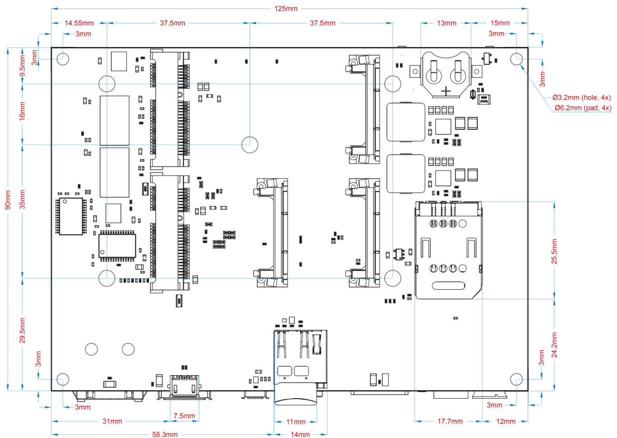
Fig.7 Ixora Carrier Board Mechanical Drawing – Bottom Side (All dimensions in millimeter)
