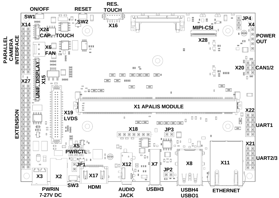
Fig.2 Ixora Carrier Board Connectors – Top Side
