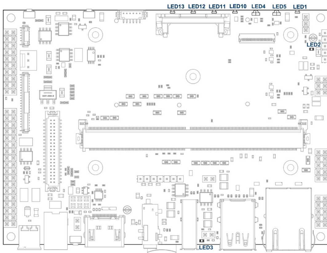
Figure 6: Indicator LEDs
