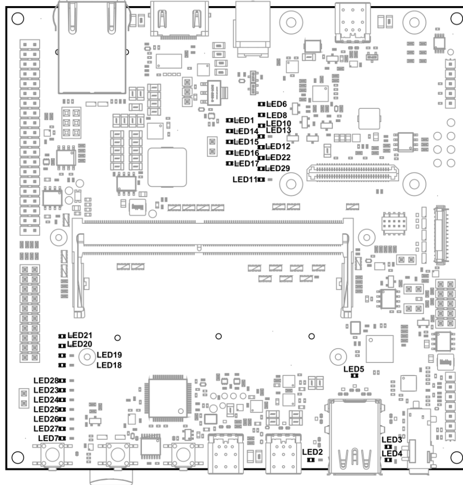
Figure 7. Indicator LEDs
