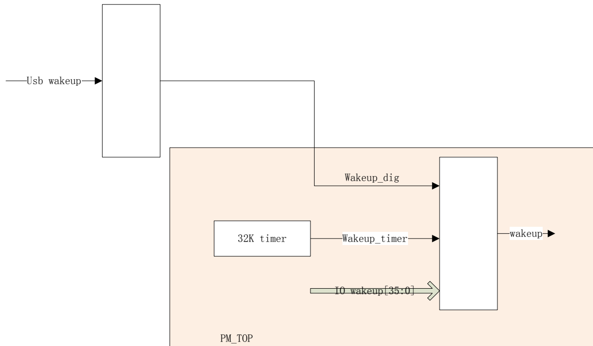
Figure 2- 6 Wakeup sources
