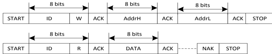
Figure 7- 4 Read format in DMA mode
