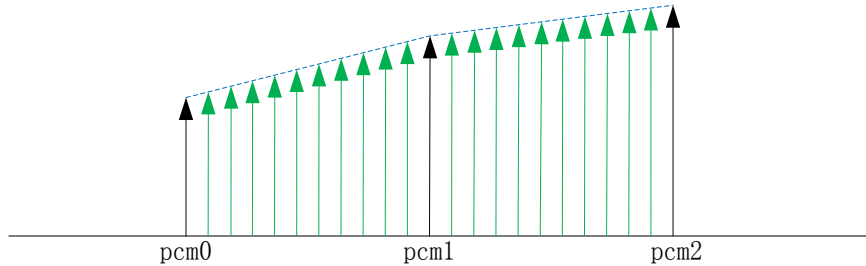
Figure 9- 4 Linear interpolation
