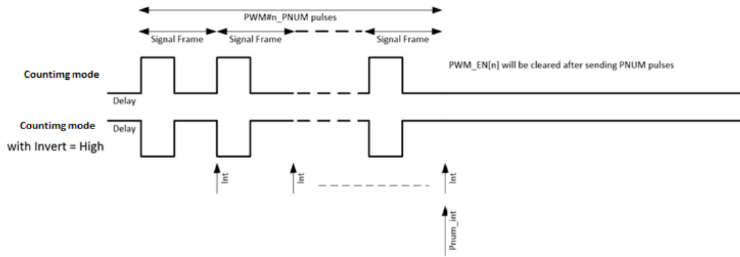
Figure 8-3 Counting mode
