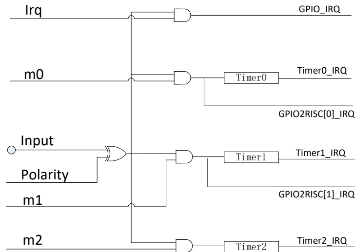
Figure 7- 2 Logic relationship between GPIO and related modules
