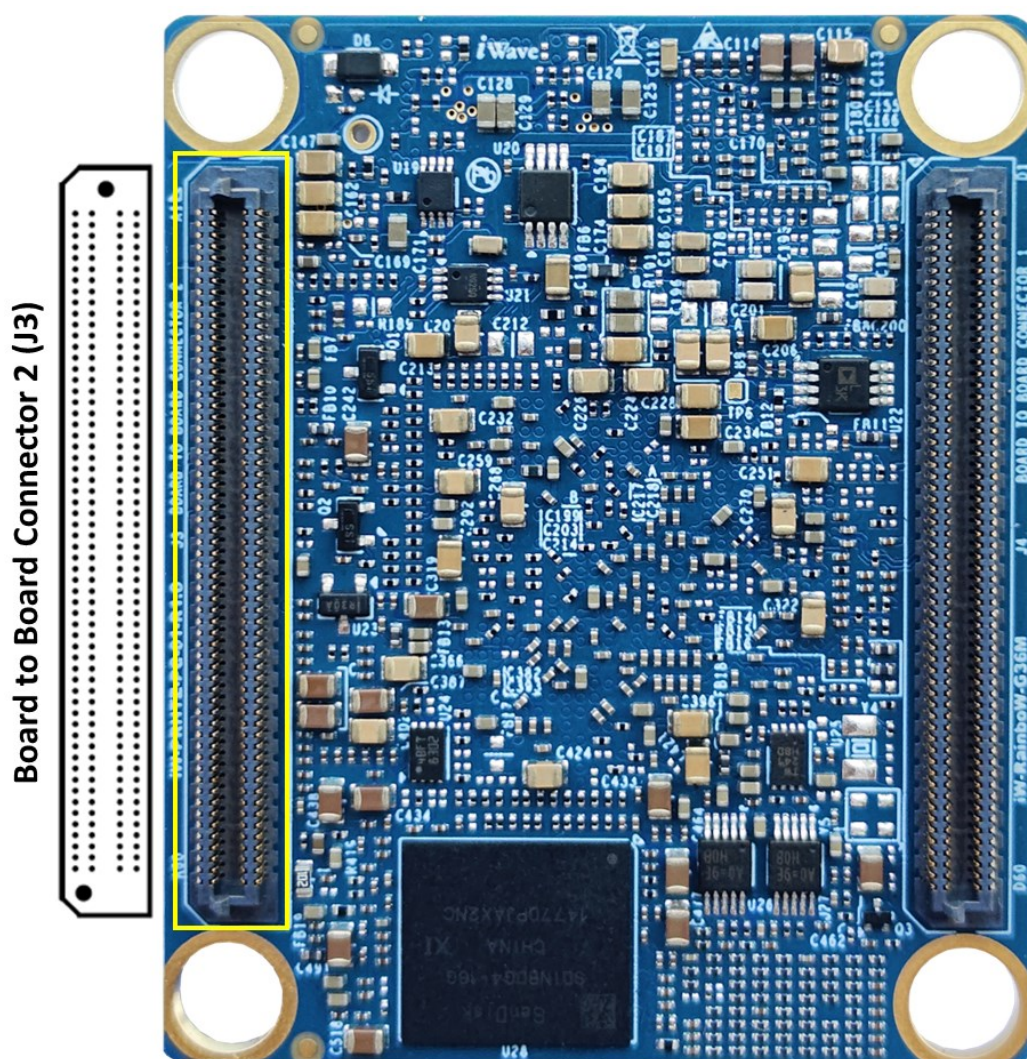
Figure 7: Board-to-Board Connector 2
