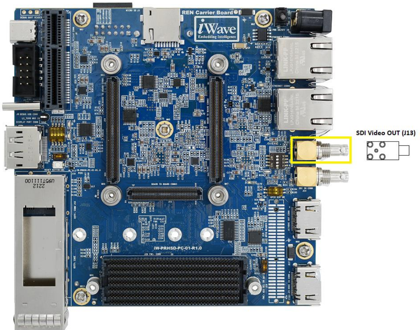
Figure 11: SDI Video OUT
