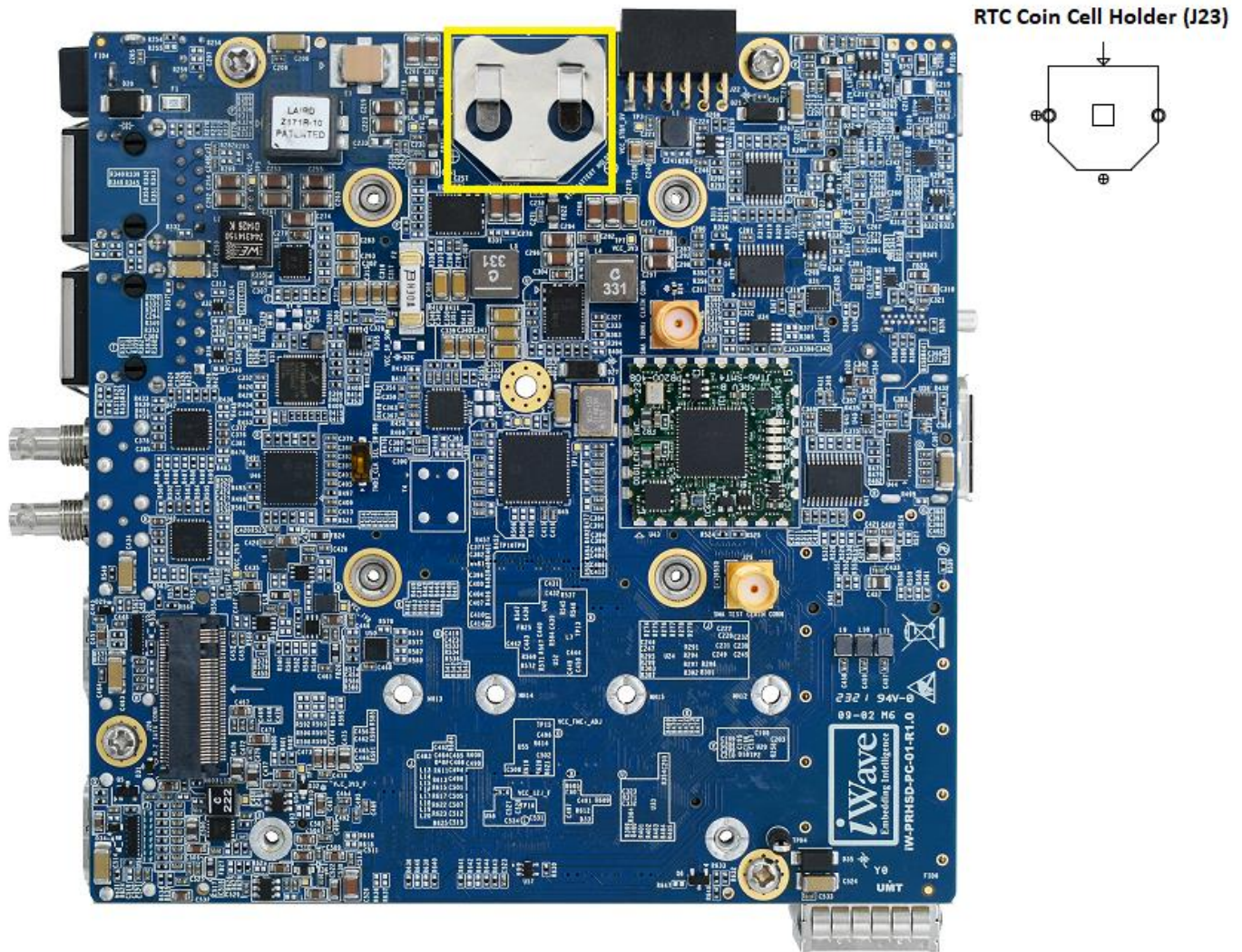
Figure 21: RTC Coin Cell Holder
