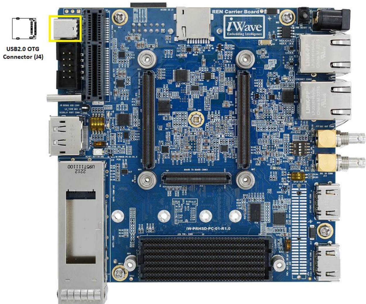
Figure 6: USB OTG Connector
