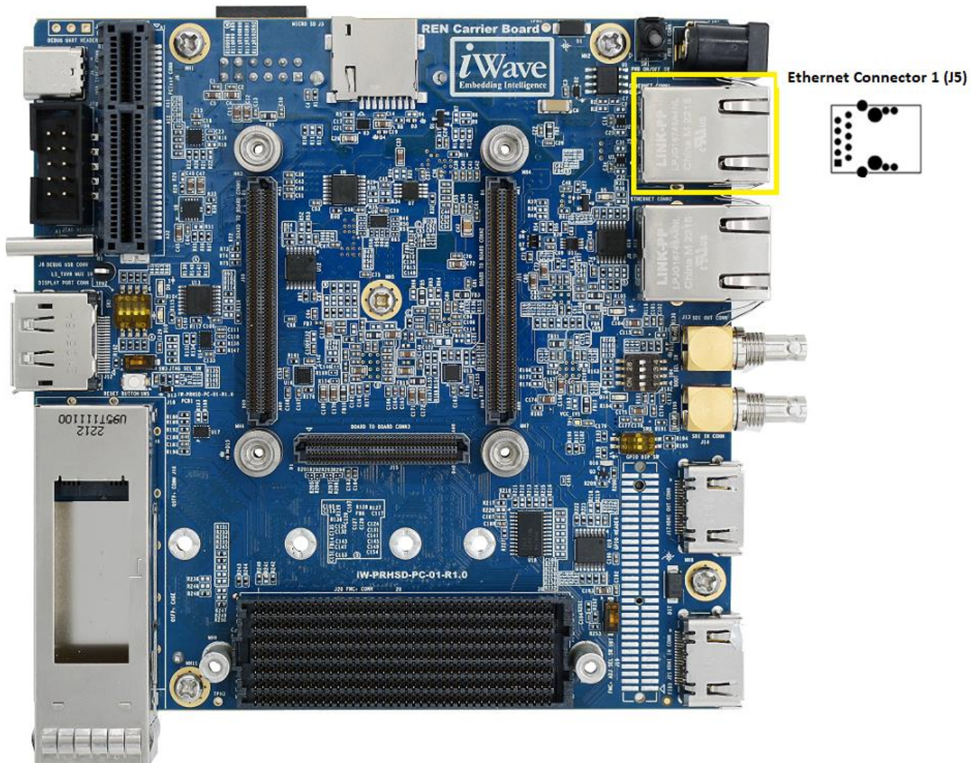
Figure 4: Gigabit Ethernet Connector1
