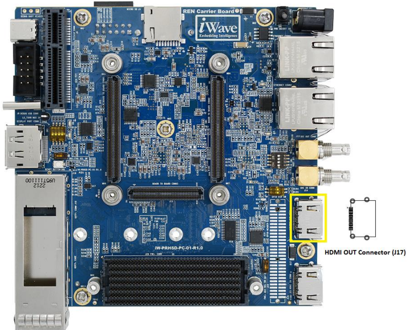
Figure 13: HDMI OUT Connector
