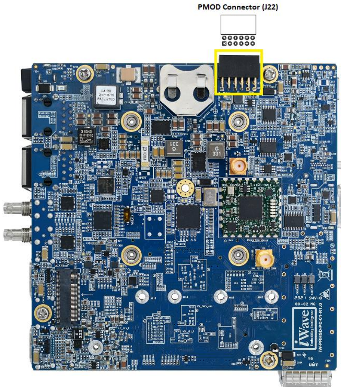
Figure 14: PMOD Host Connector
