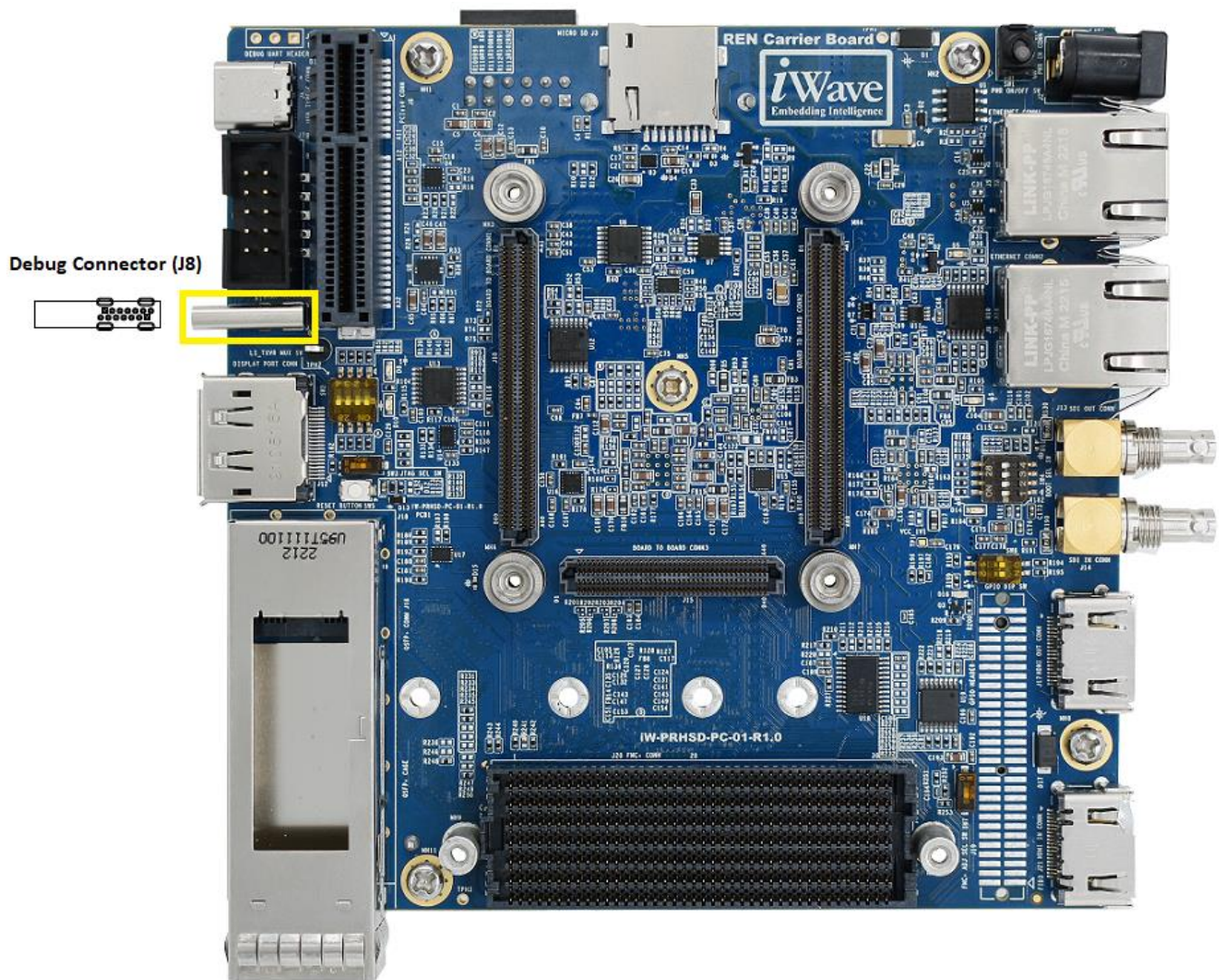
Figure 9: Debug Connector
