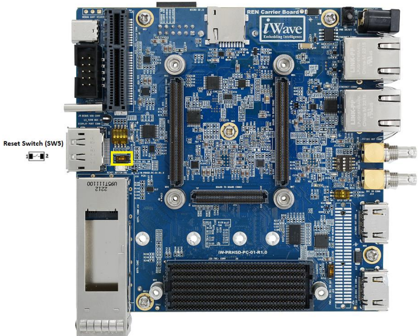
Figure 20: Reset Switch
