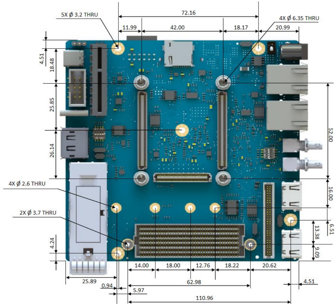
Figure 23: Carrier board Mechanical dimension – Top View
