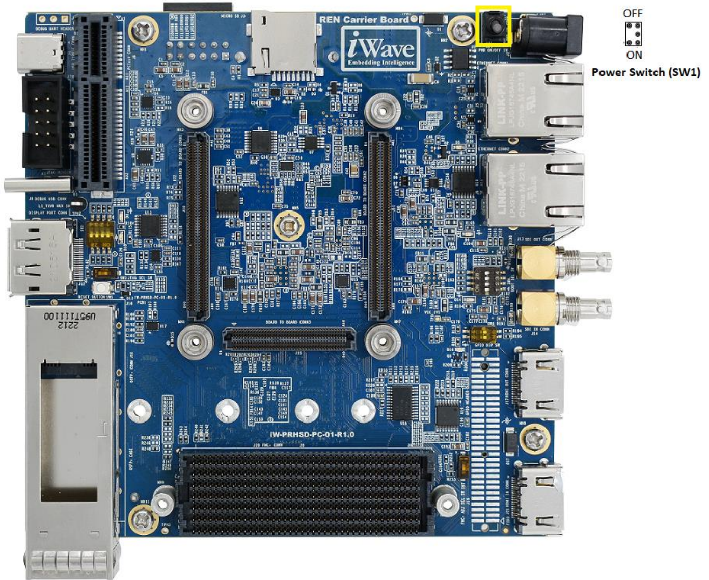
Figure 19: Power On/Off Switch
