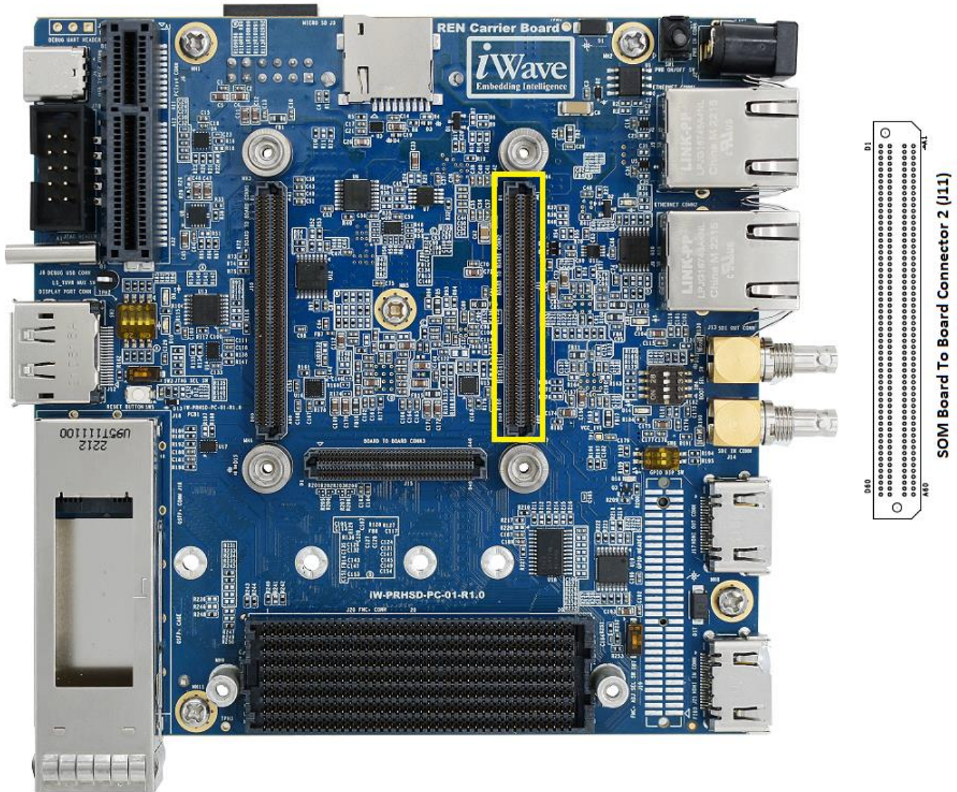
Figure 3: Board to Board Connector 2
