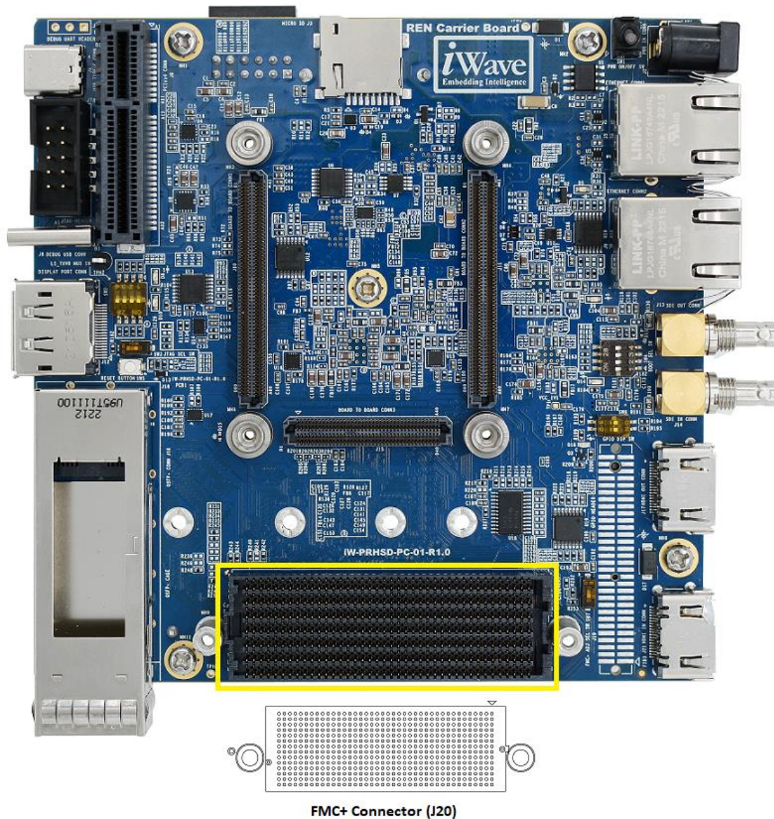
Figure 15: FMC+ Connector
