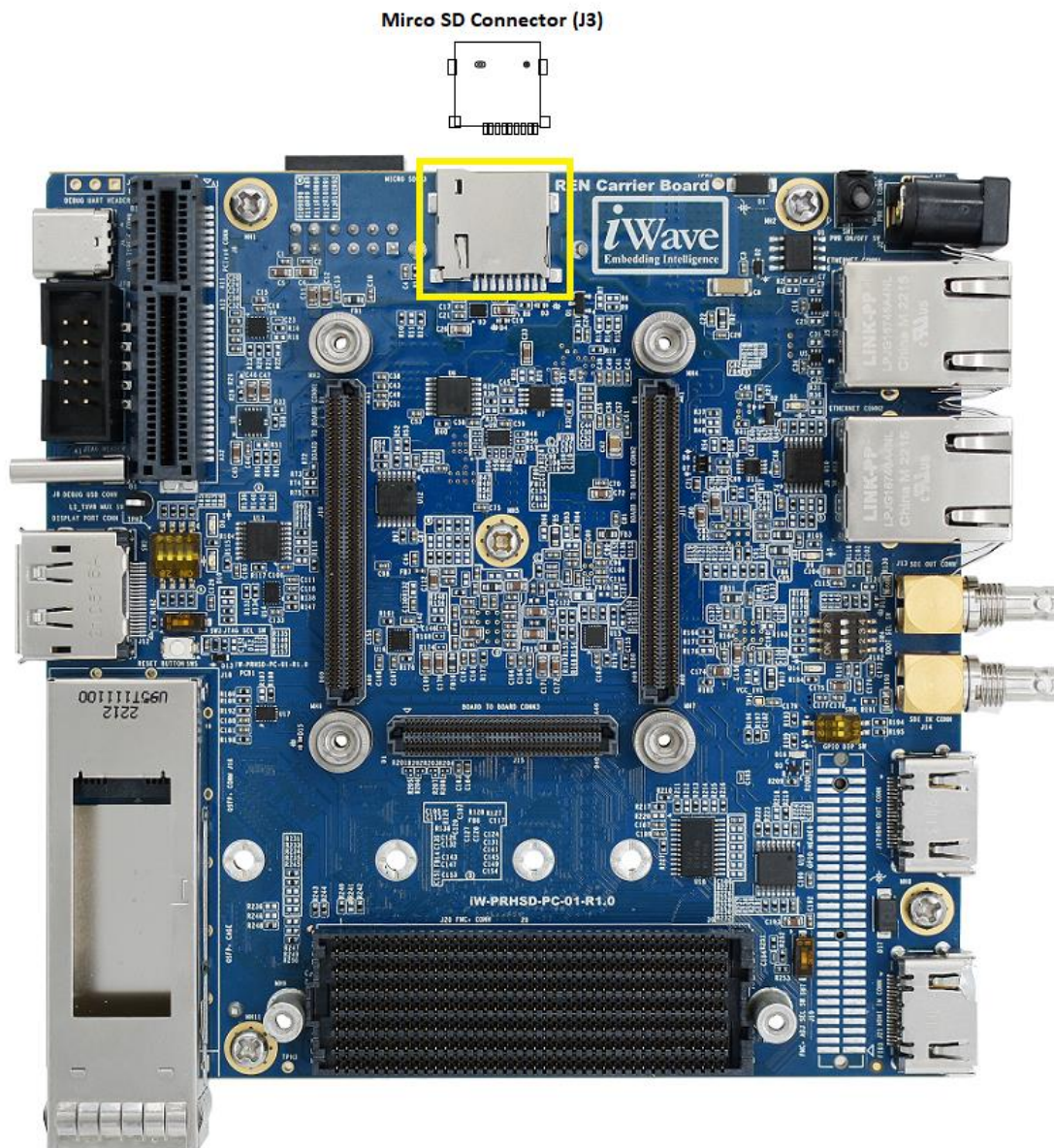
Figure 7: Micro SD Connector
