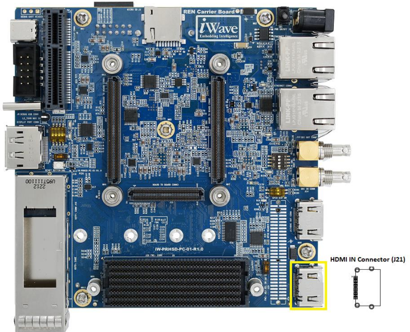
Figure 12: HDMI IN Connector
