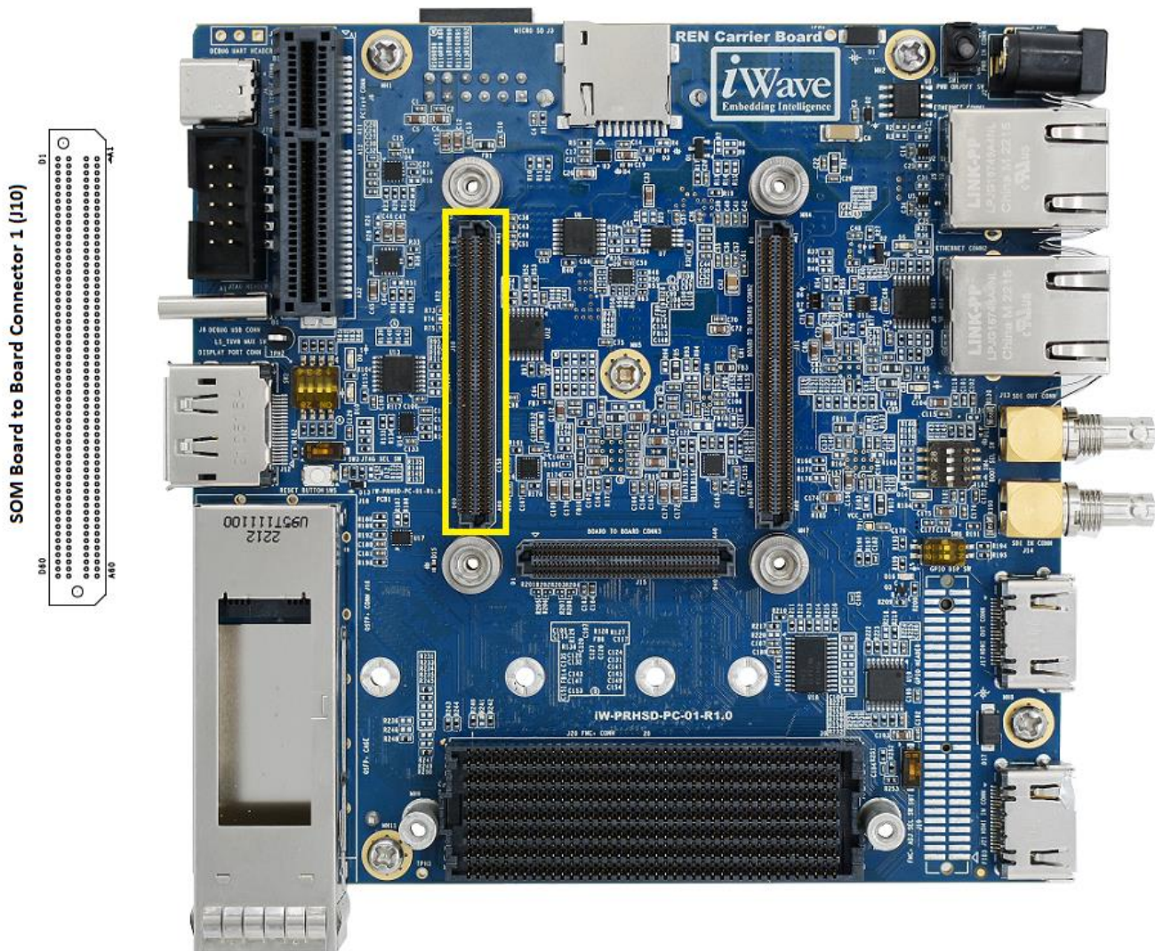
Figure 2: Board to Board Connector1
