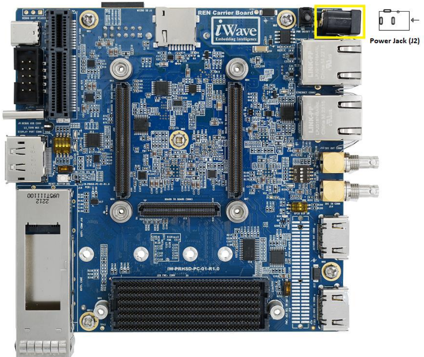
Figure 22: Power Jack
