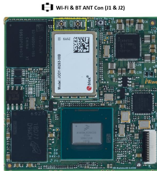
Figure 3: Wi-Fi and Bluetooth Antenna Connector
