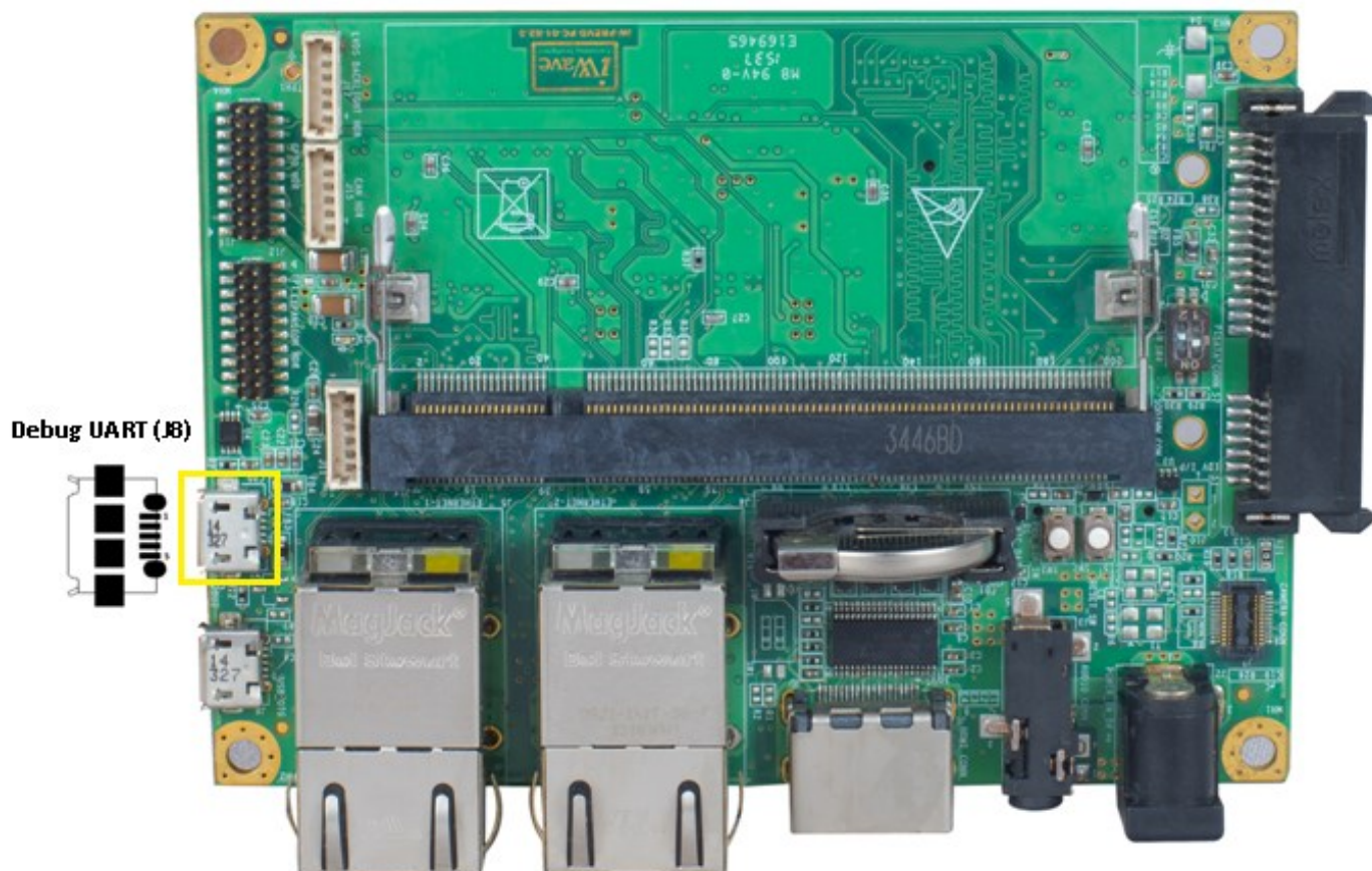
Figure 3: Debug UART
