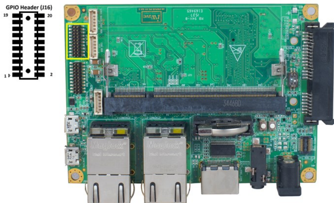
Figure 20: GPIO Header
