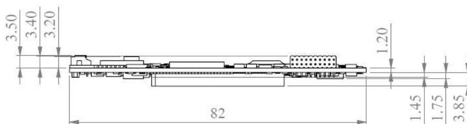
Figure 11: Mechanical dimension of i.MX8M SMARC SOM- Side View
