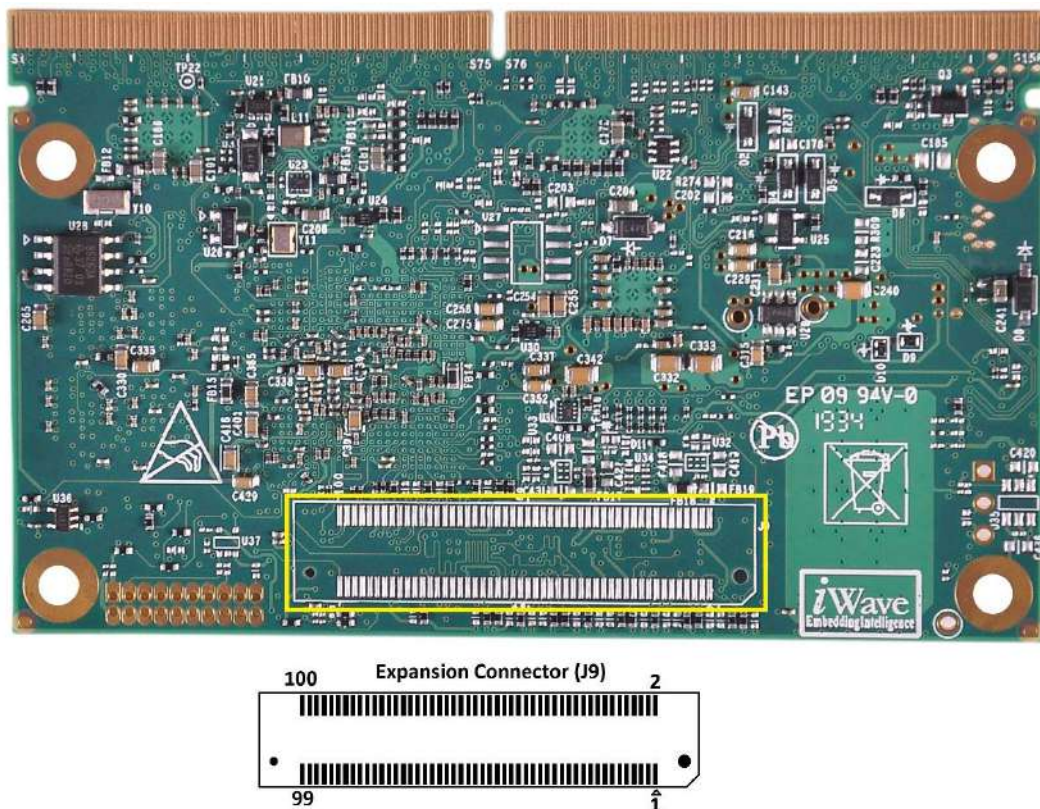
Figure 5: Expansion Connector
