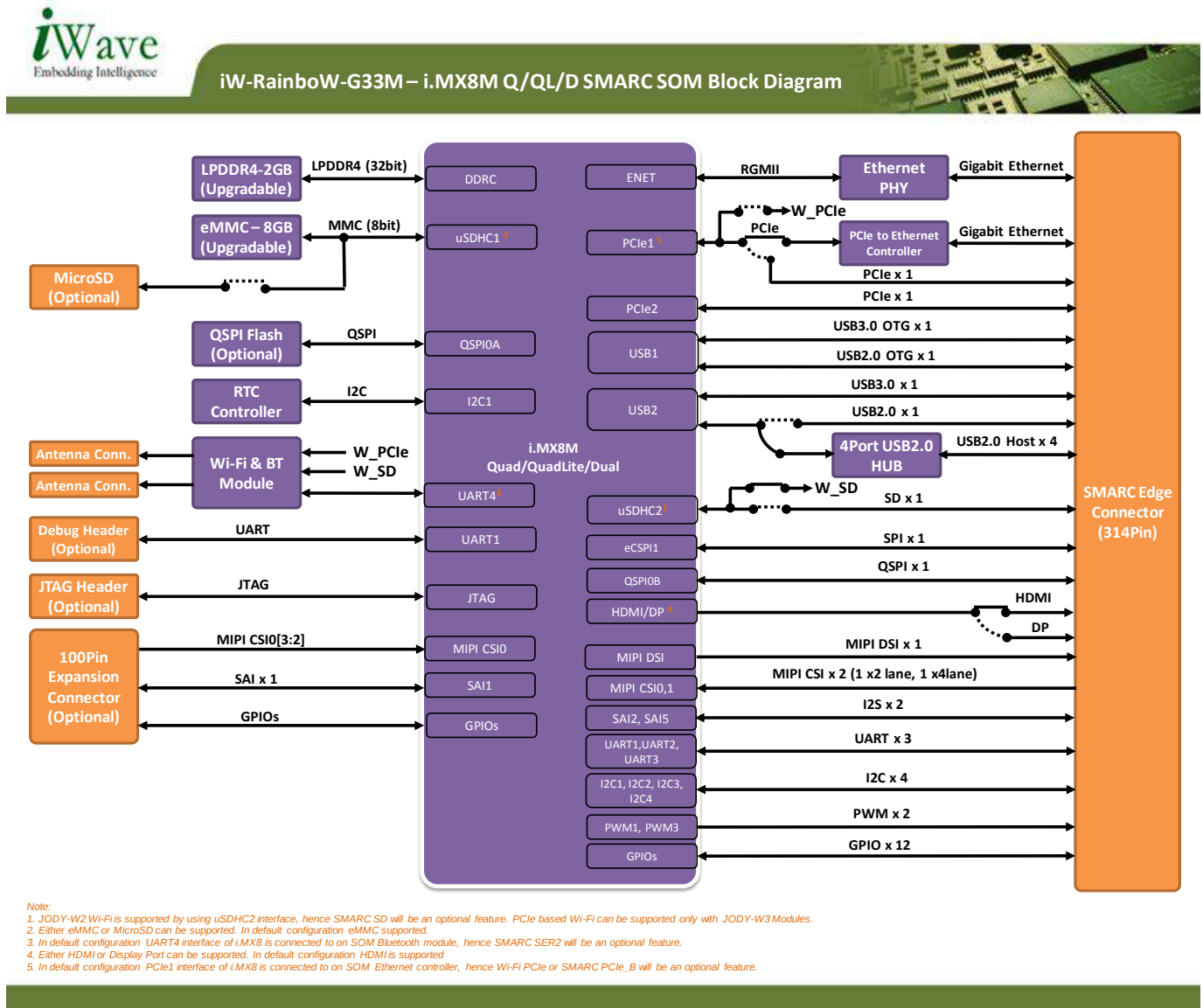
Figure 1: i.MX8M SMARC SOM Block Diagram
