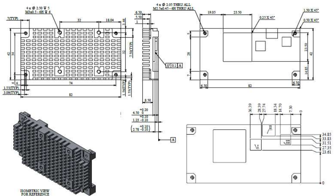
Figure 9: Heat Sink Dimension
