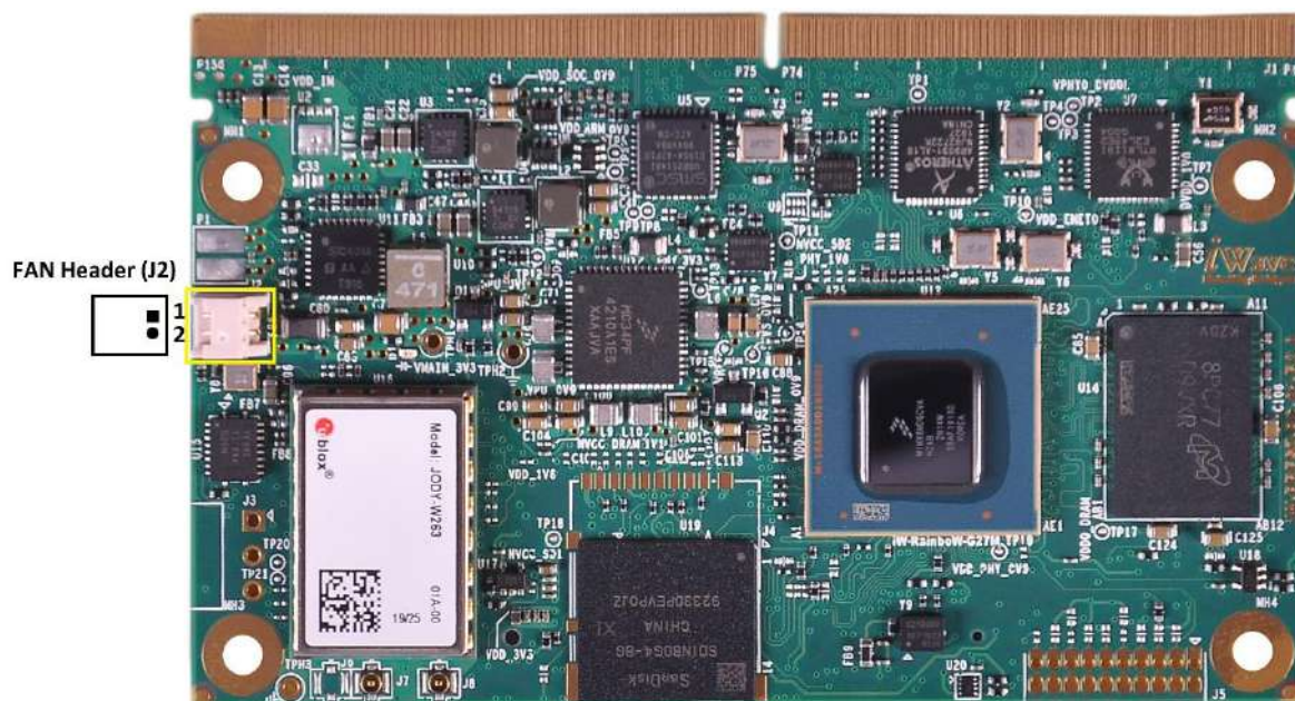
Figure 6: FAN Header
