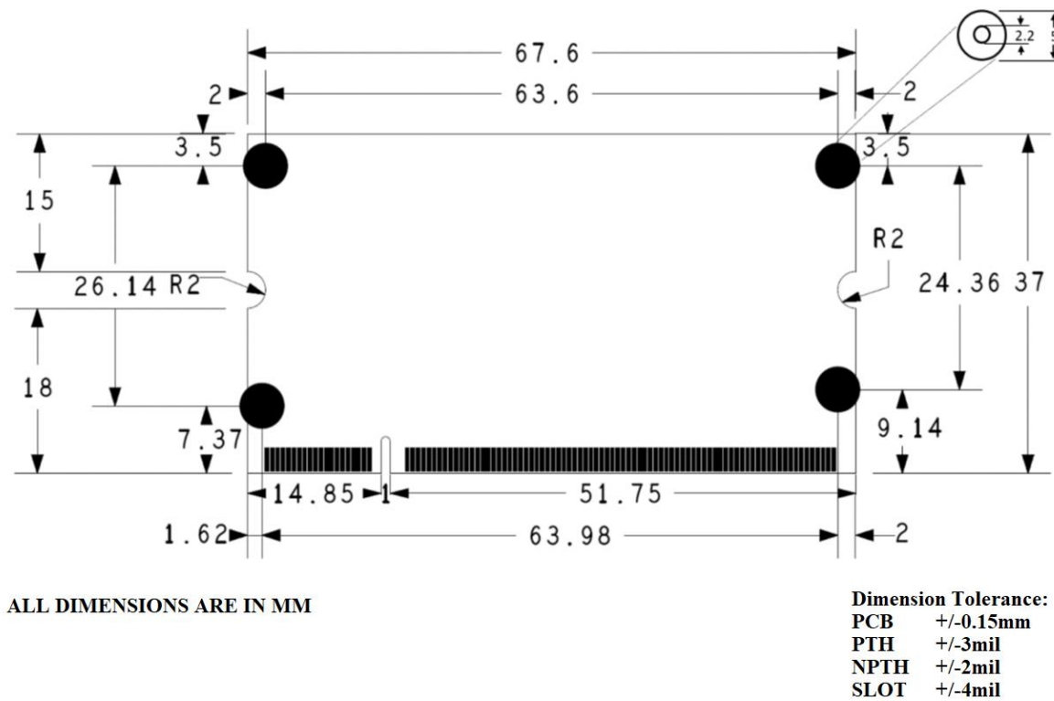
Figure 7: Mechanical dimension of Zynq-7000 SoC SODIMM SOM - Top View
