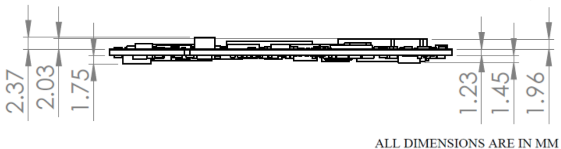
Figure 8: Mechanical dimension of Zynq-7000 SoC SODIMM SOM- Side View
