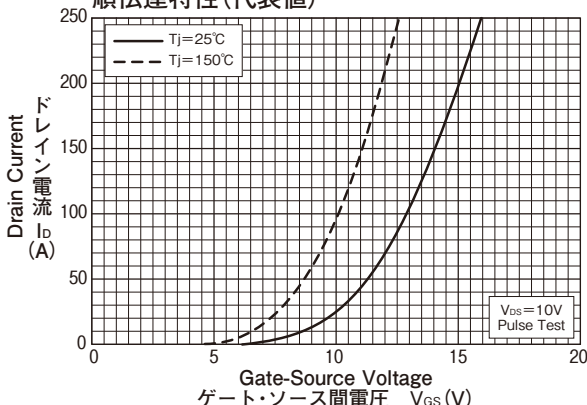
Forward Transfer Characteristics (Typical) 順伝達特性 (代表値)
